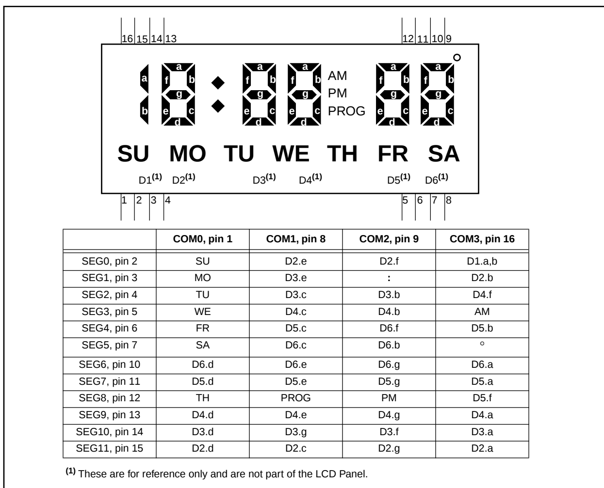
Figure 8.3 Pixel Layout
