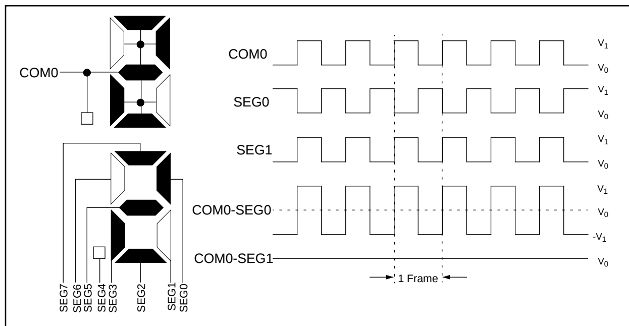
Figure 3.19 STATIC Waveforms
