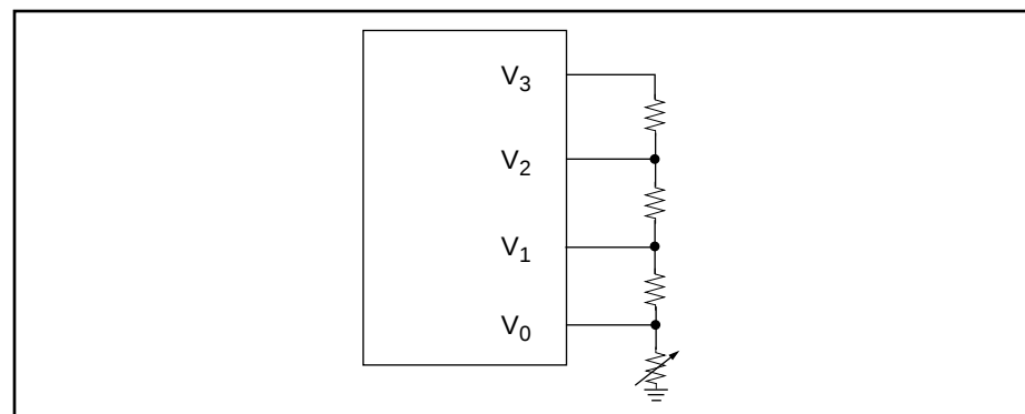
Figure 3.23 Resistor Ladder
