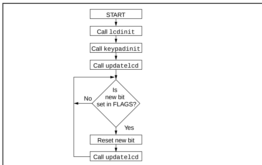
Figure 5.1 Main Routine Block Diagram
