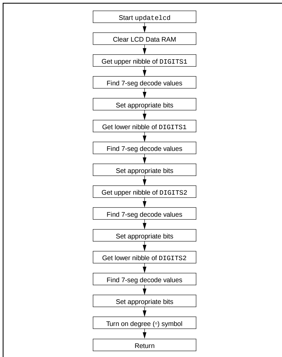
Figure 6.7 update1cd Routine Block Diagram
