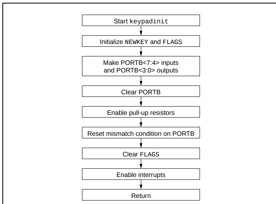
Figure 5.4 keypadinit Block Diagram
