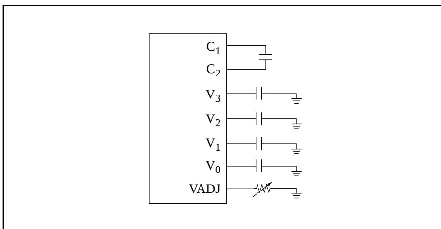
Figure 3.25 Charge Pump
