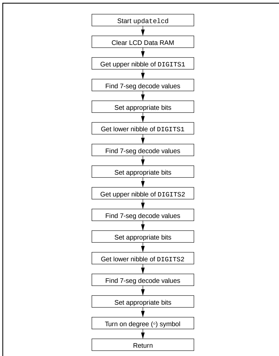
Figure 4.3 update1cd Block Diagram
