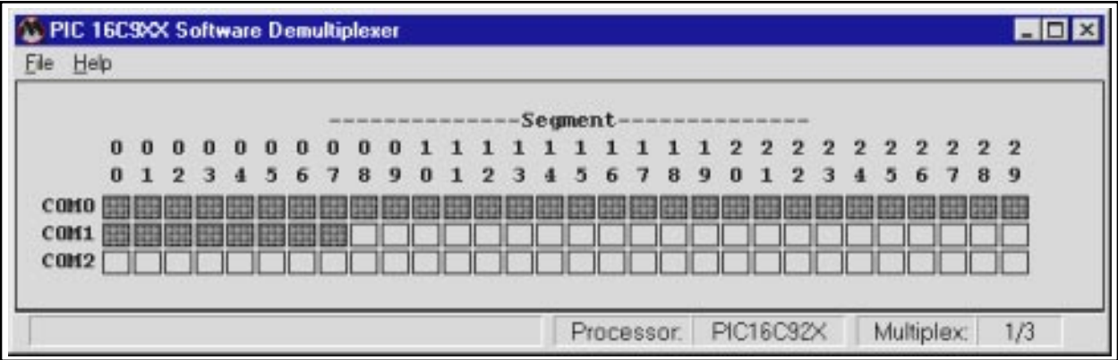
Figure 2.4 1/3 MUX
