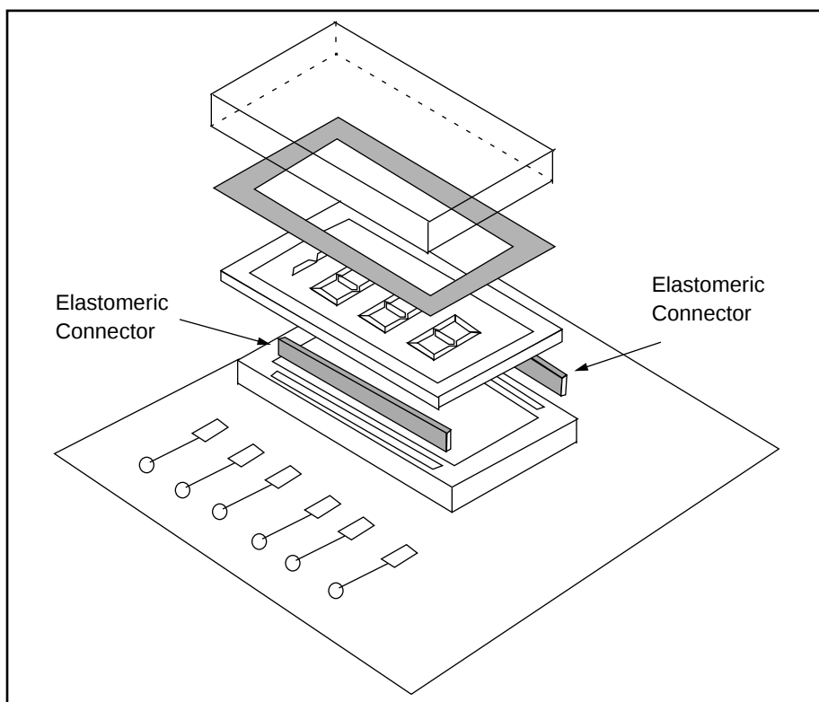
Figure 3.13 Elastomeric Connectors
