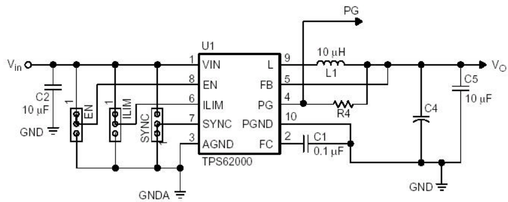
Figure 1–2. TPS62005 and TPS62007 (SLVS169) EVM Schematic Diagram
