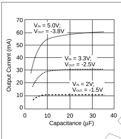
Figure 7. Output Current vs. Capacitance for the SP828
