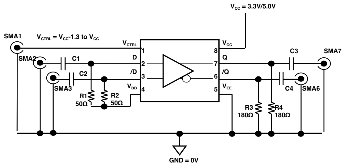
SY89307V AC-Coupled Evaluation Board
