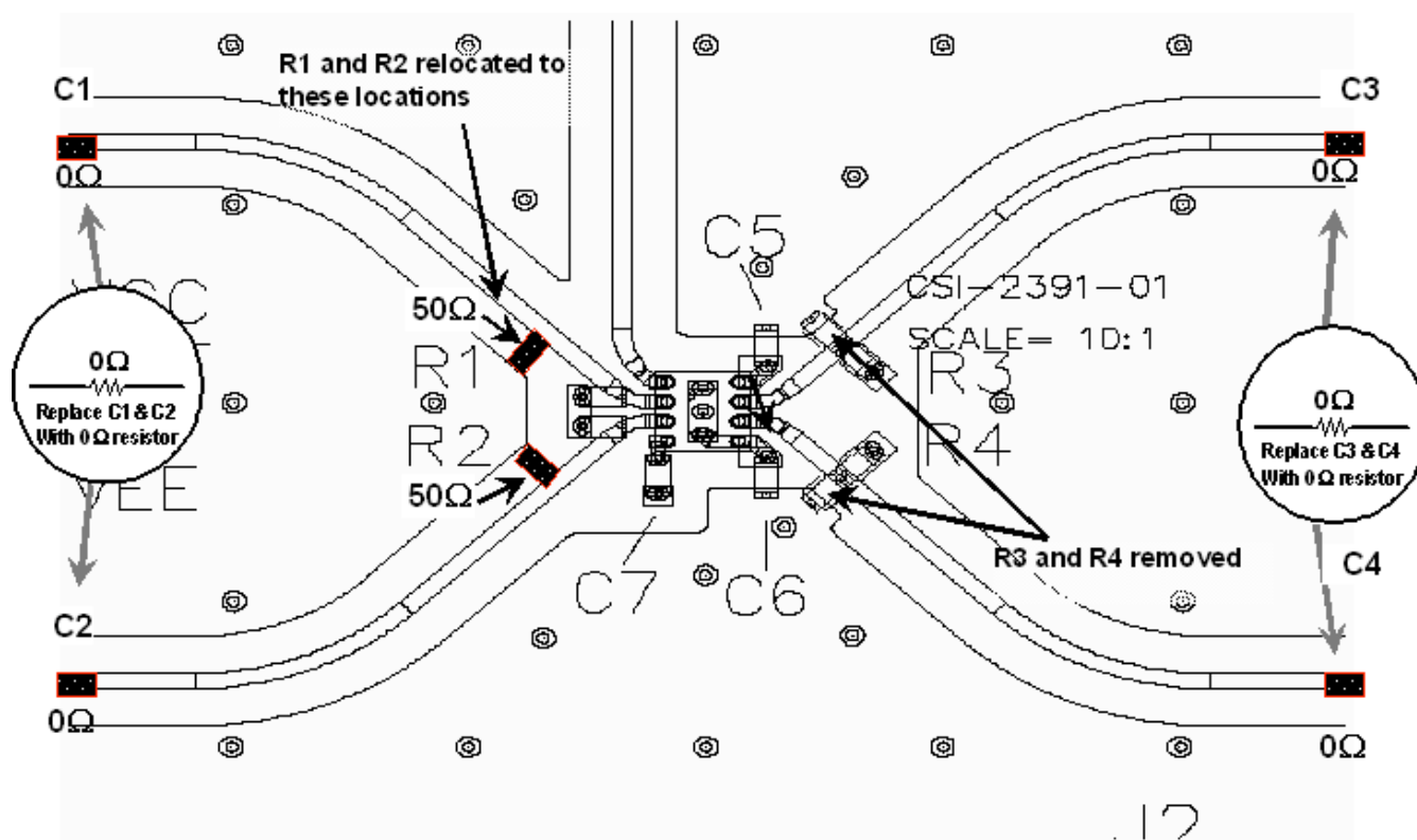
SY89307V DC-Coupled Loading Diagram
