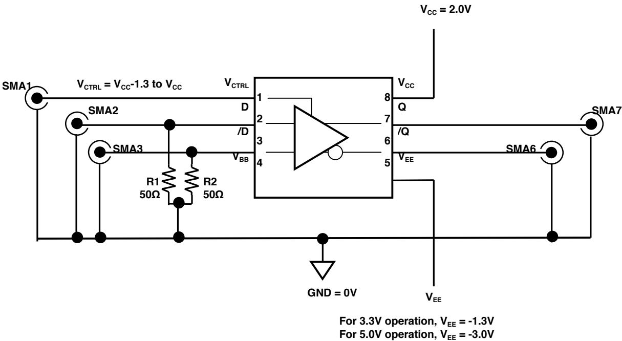
SY89307V DC-Coupled Evaluation Board
