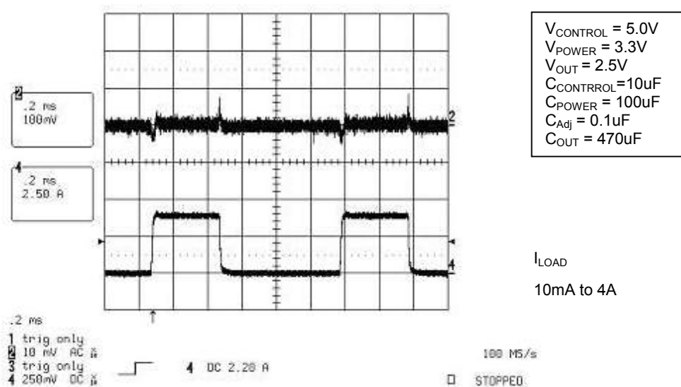
Transient Response
