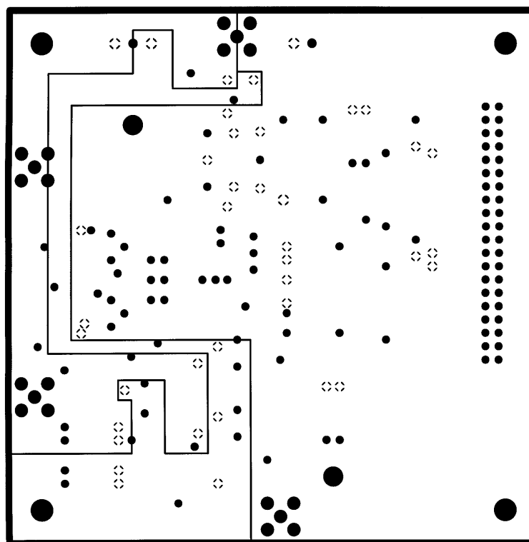
FIGURE 3. Power Plane; DEM-ADS8xxU.
