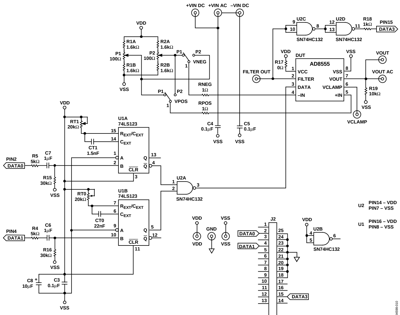
Figure 14. Evaluation Board Schematic
