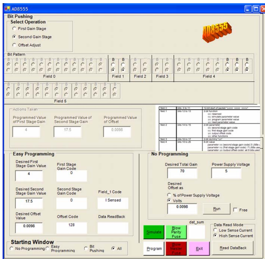
Figure 6. AD8555 Dialog Box with All Modes Displayed
