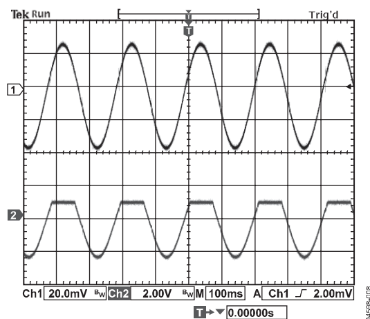
Figure 12. Response with V_{CLAMP} Set
