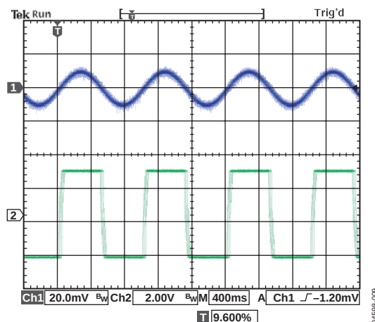
Figure 13. Results with Saturation
