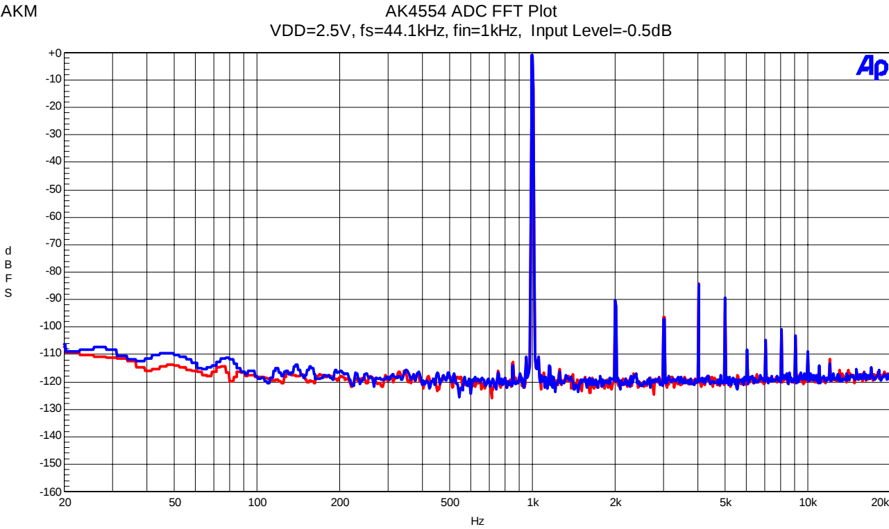
Fig.5 FFT Plot (Input Level = -0.5dB)
