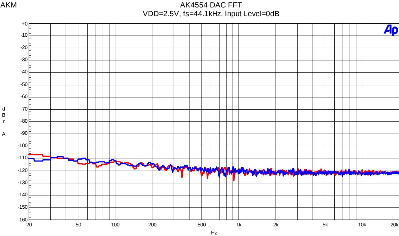
Fig.15 FFT Plot (no data)
