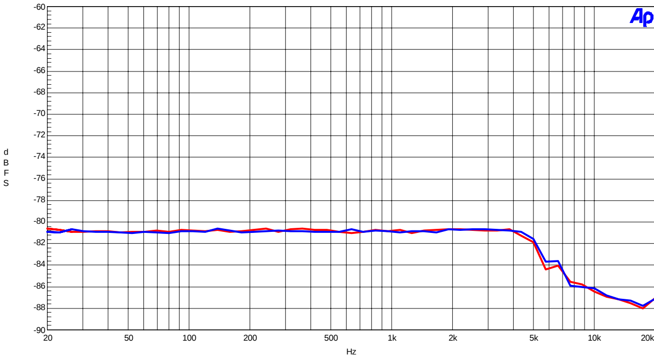
Fig.2 THD+N vs. Input Frequency
