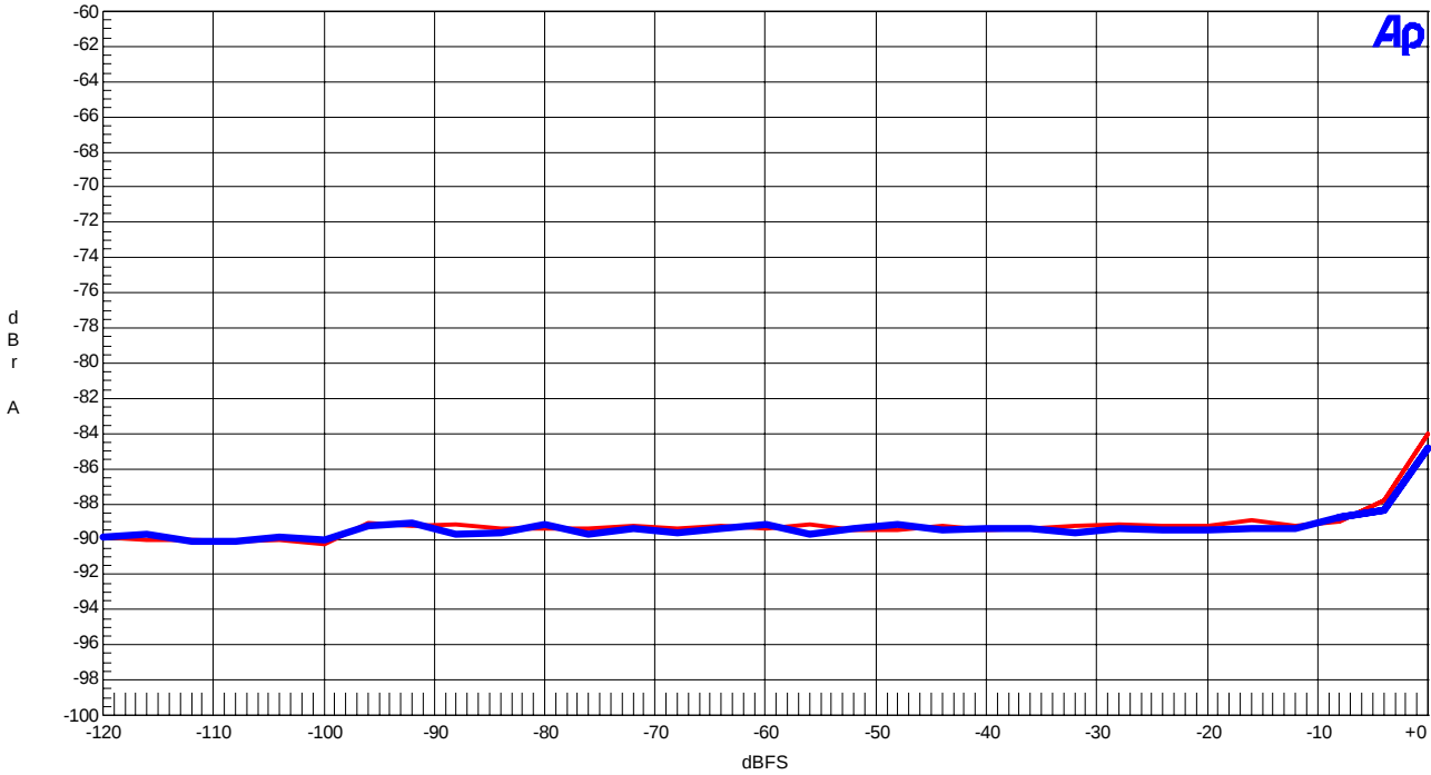
Fig.9 THD+N vs. Input Level
