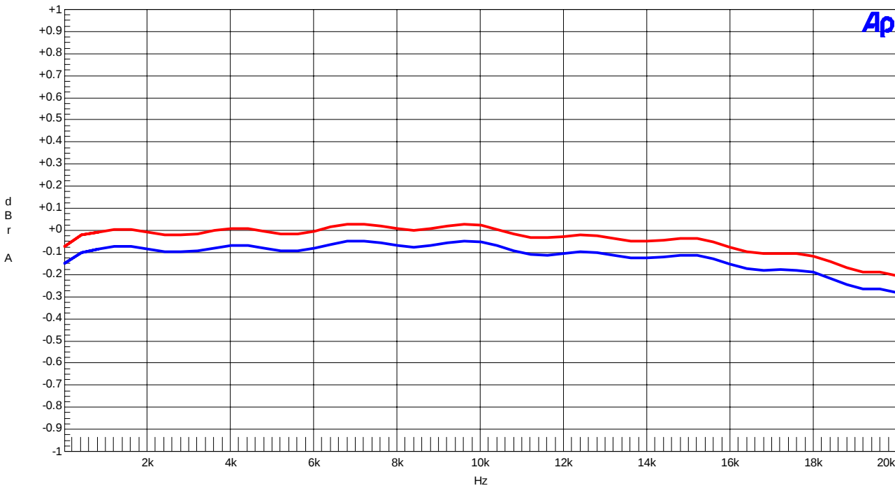
Fig.12 Frequency Response
