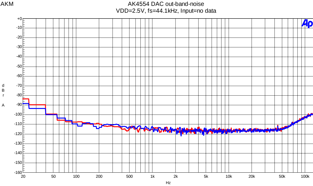
Fig.17 Out band noise
