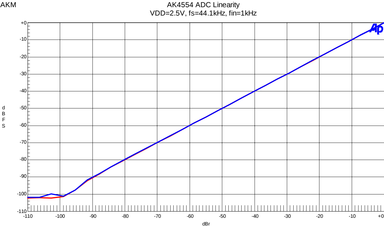
Fig.3 Linearity
