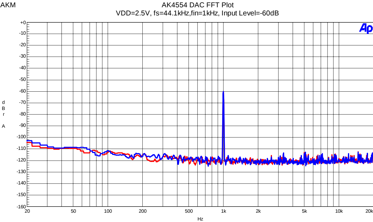
Fig.14 FFT Plot (Input Level = -60dB)
