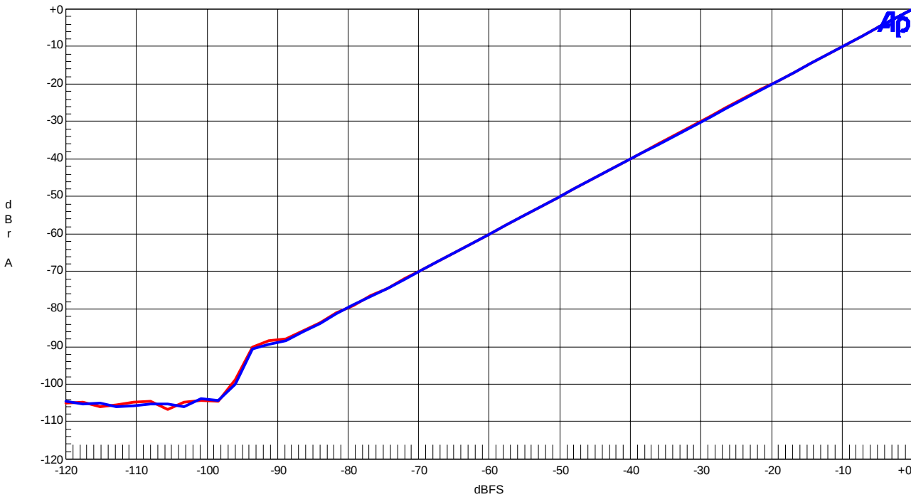
Fig.11 Linearity
