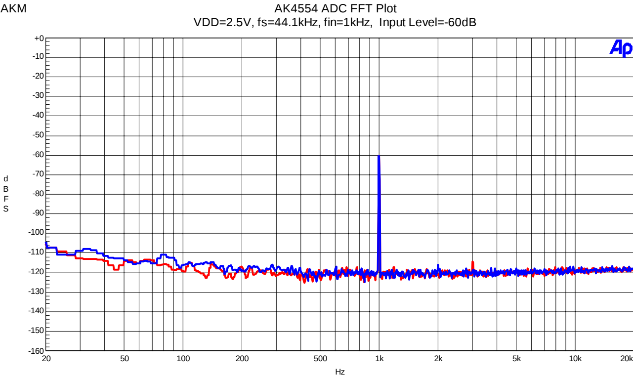
Fig.6 FFT Plot (Input Level = -60dB)
