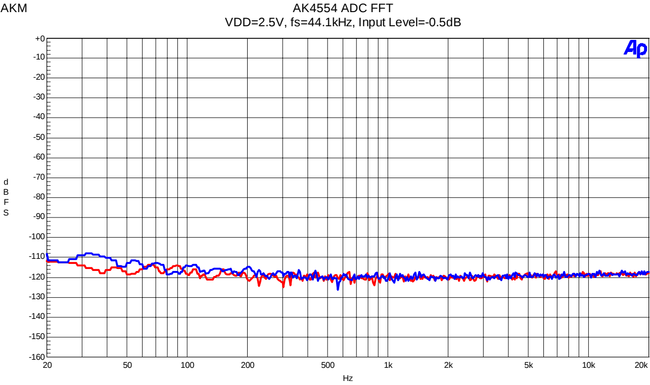
Fig.7 FFT Plot (no signal)
