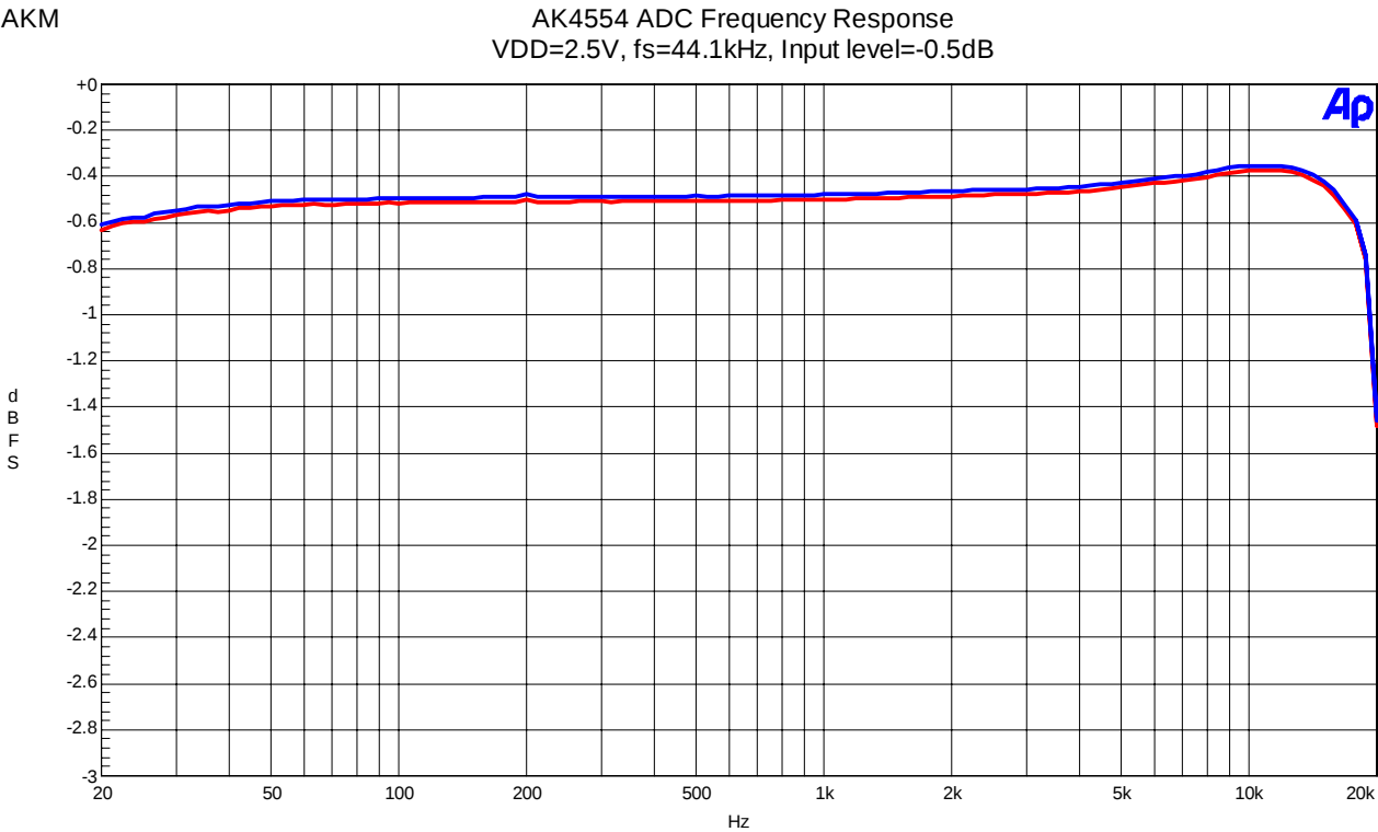
Fig.4 Frequency Response
