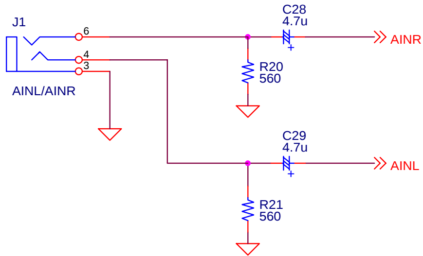
Figure 2. Input circuit on board
