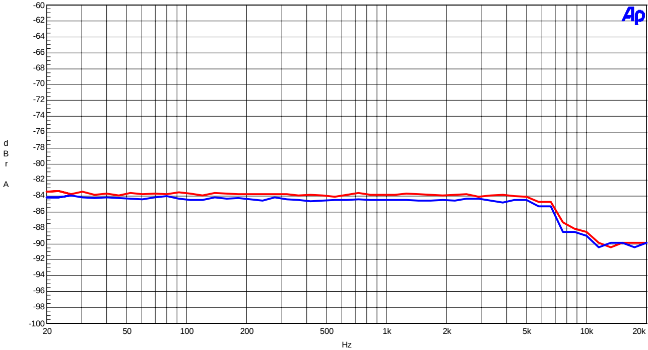
Fig.10 THD+N vs. Input Frequency
