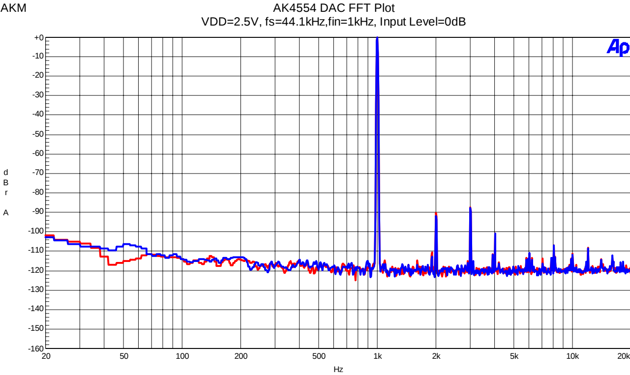
Fig.13 FFT Plot (Input Level = 0dB)
