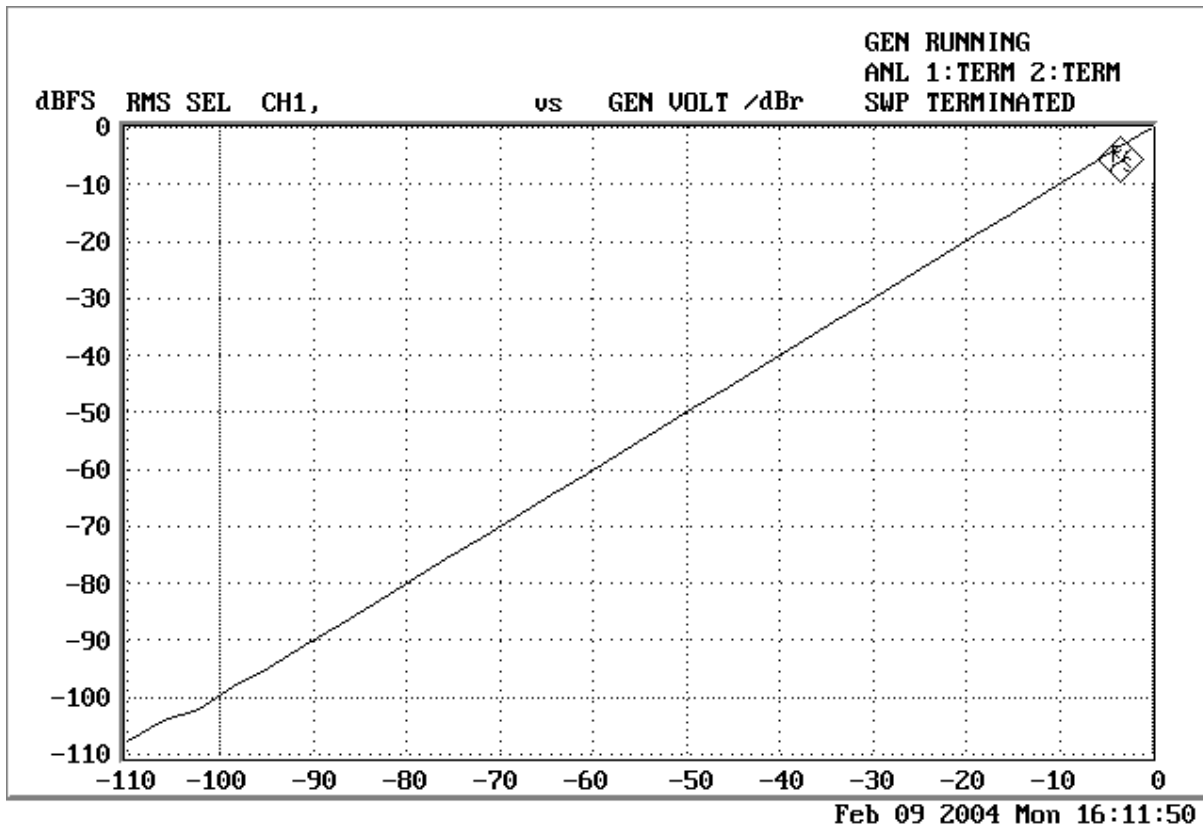
Figure 10. Linearity
