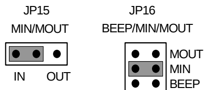
Figure 6. BEEP/MIN/MOUT Input and Output Circuit
