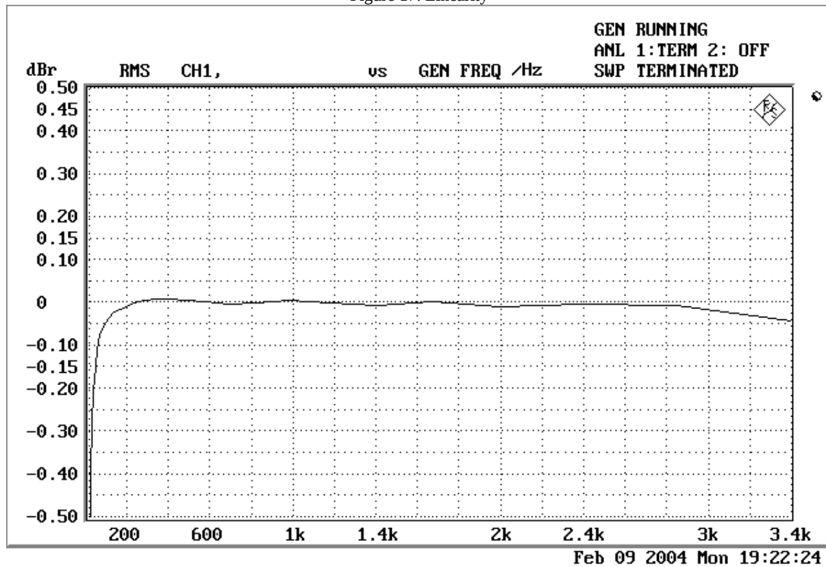
Figure 18. Frequency Response
