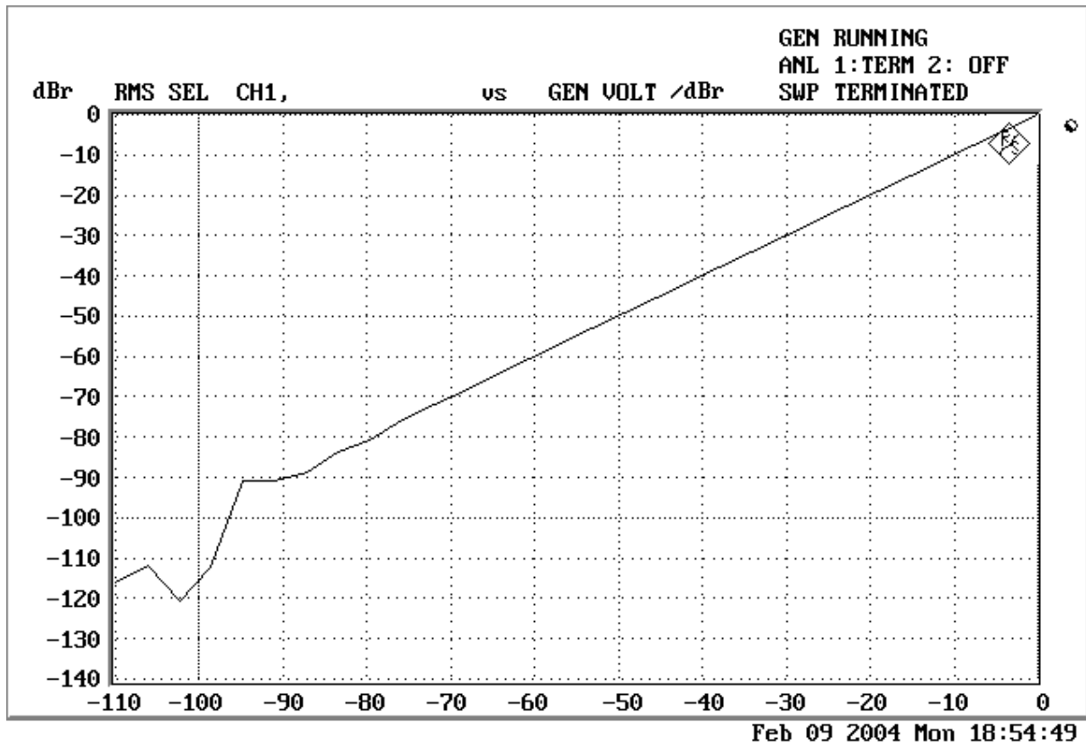
Figure 17. Linearity
