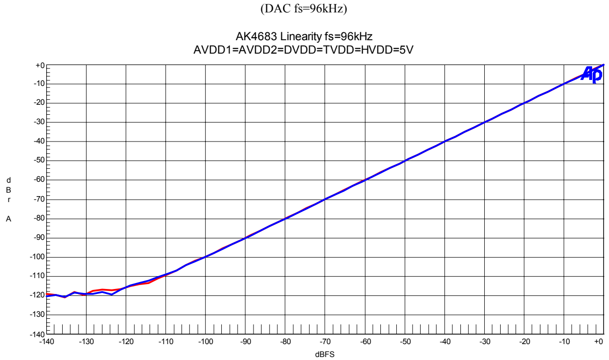
Figure 41. Linearity (Input Frequency = 1kHz)
