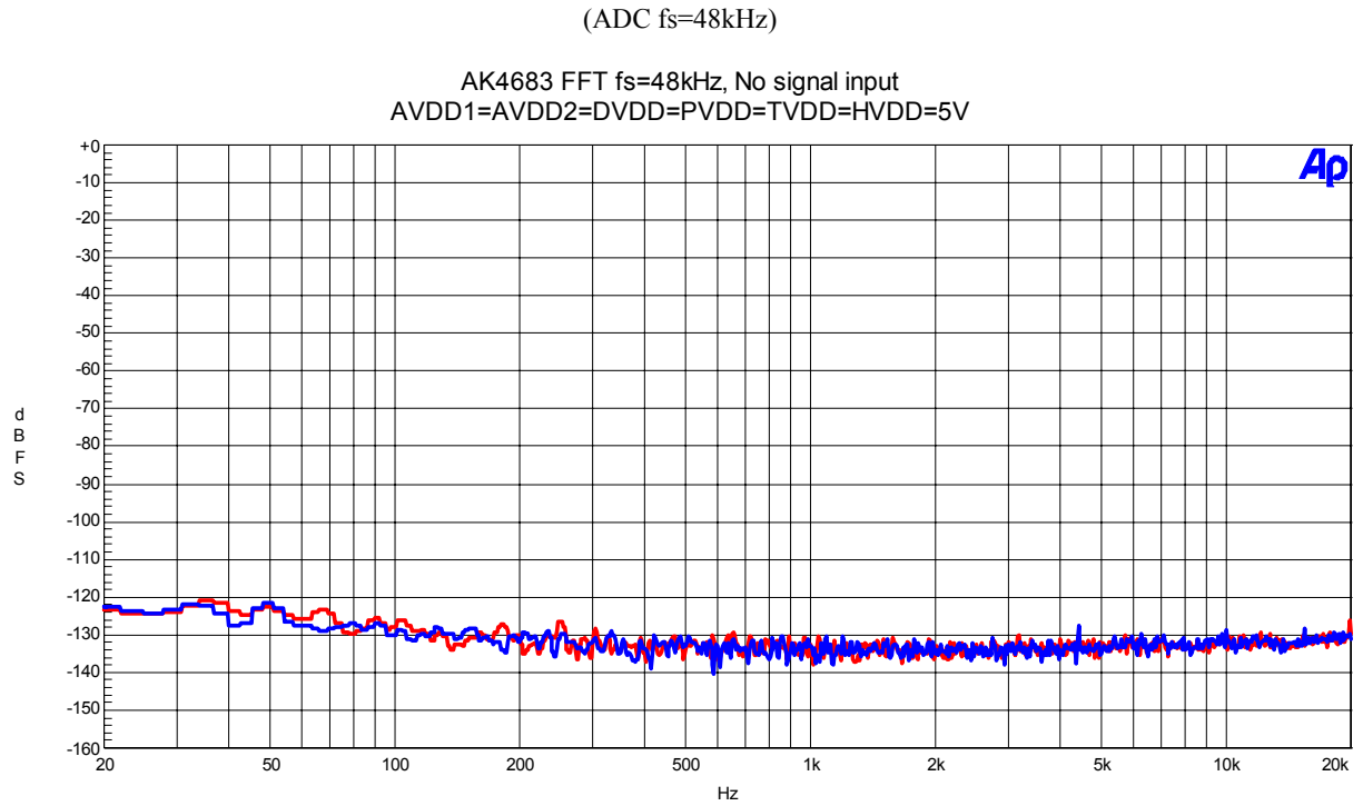
Figure 12. FFT(noise floor)
