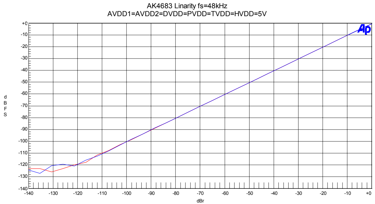
Figure 15. Linearity (Input Frequency =1kHz)
