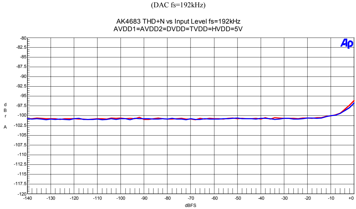
Figure 48. THD+N vs Input Level (Input Frequency =1kHz)
