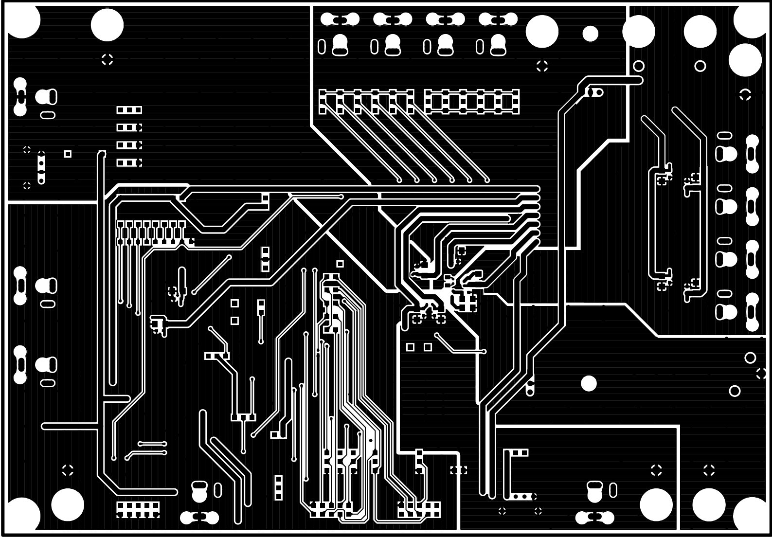
AKD4683-B JS
