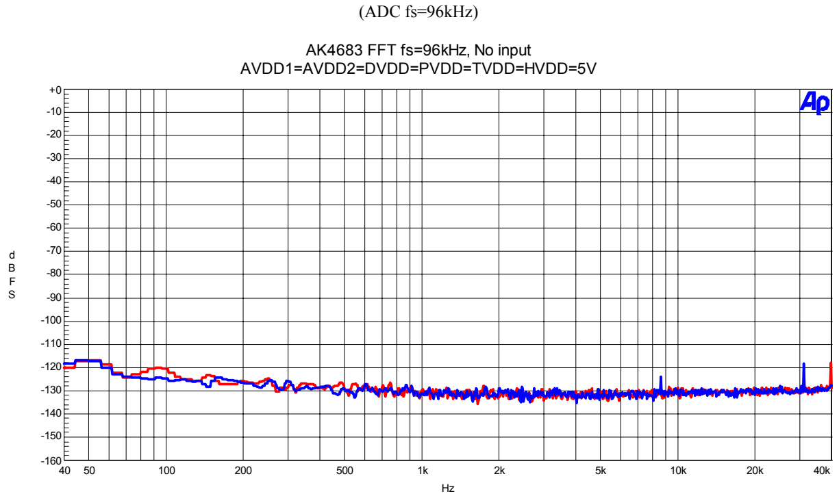
Figure 20. FFT(Noise floor)
