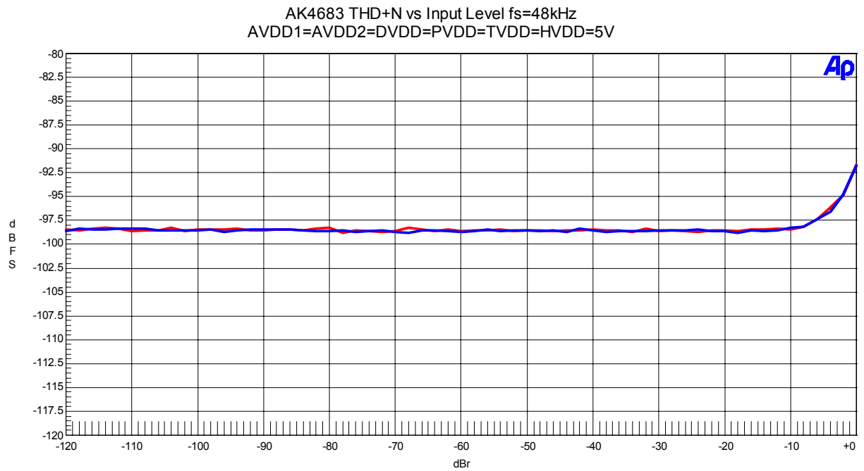
Figure 13. THD + N vs Input Level (Input Frequency =1kHz)
