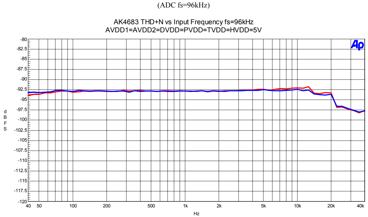
Figure 22. THD + N vs Input Frequency (Input Level=-0.5dBFS)
