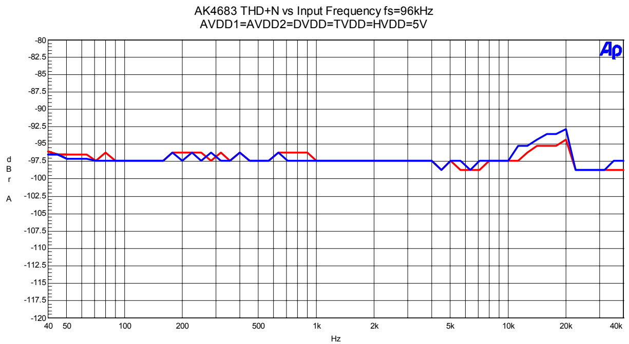
Figure 40. THD+N vs fin (Input Level=0dBFS)
