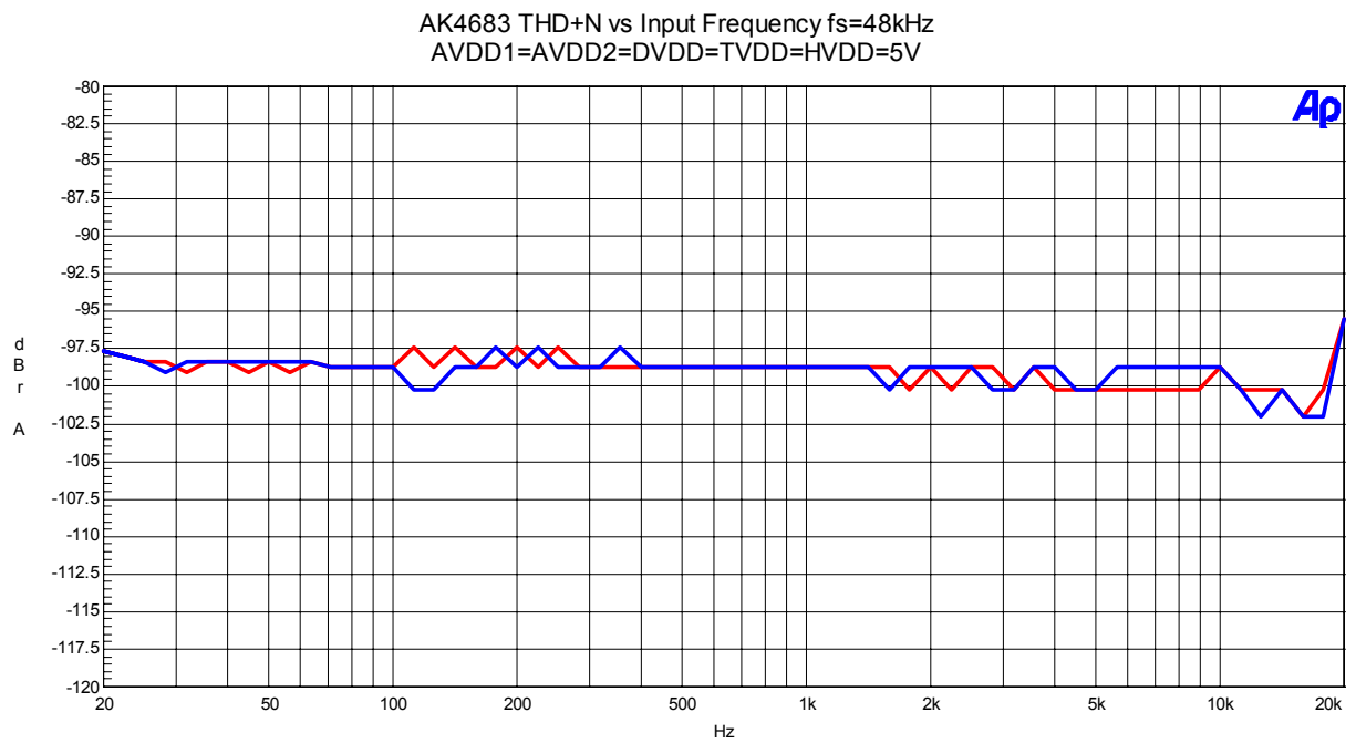
Figure 31. THD+N vs Input Frequency (Input Level=0dBFS)
