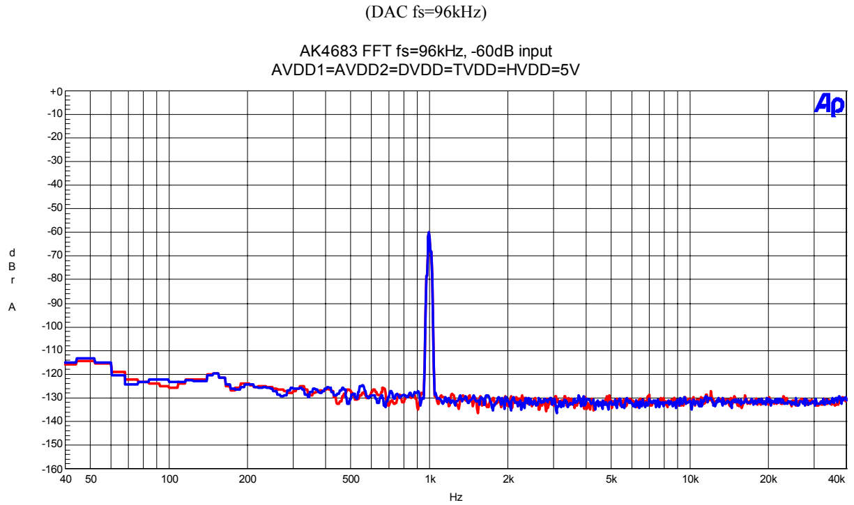
Figure 37. FFT(Input Frequency =1kHz, Input Level=-60dBFS)
