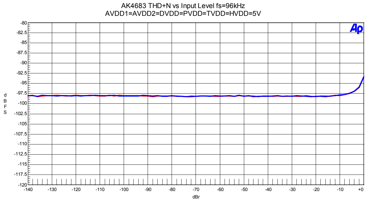
Figure 21. THD + N vs Input Level (Input Frequency =1kHz)
