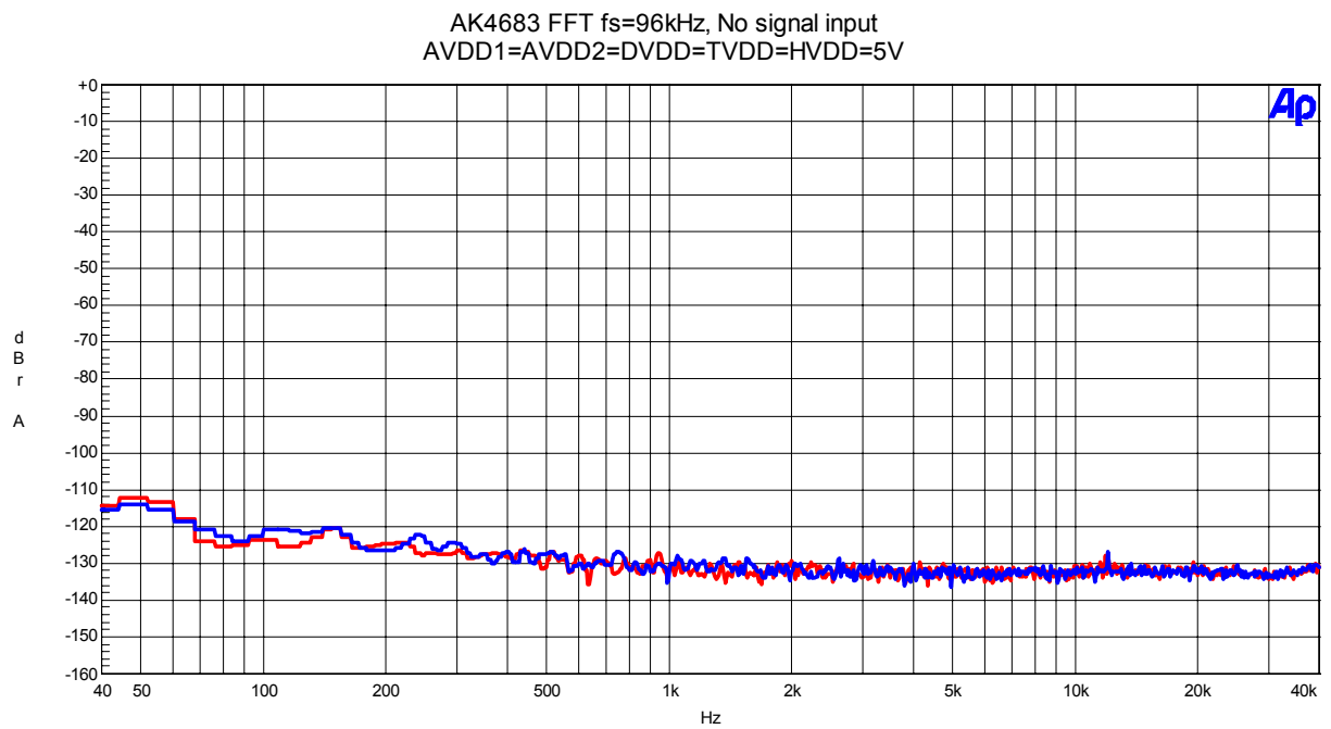
Figure 38. FFT(noise floor)
