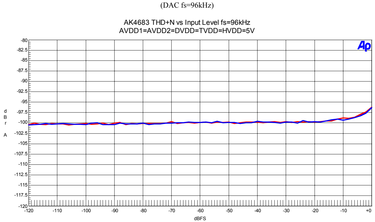
Figure 39. THD+N vs Input Level (Input Frequency =1kHz)
