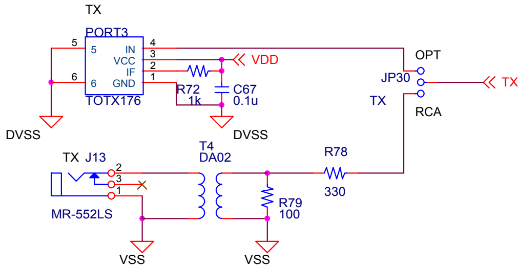
Figure 7. Digital Output Circuit (Internal DIT)
