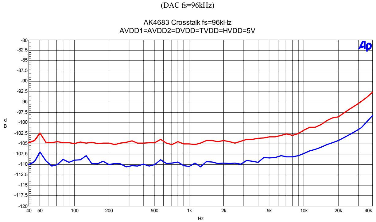
Figure 43. Cross-talk (Input Level=0dBFS)
