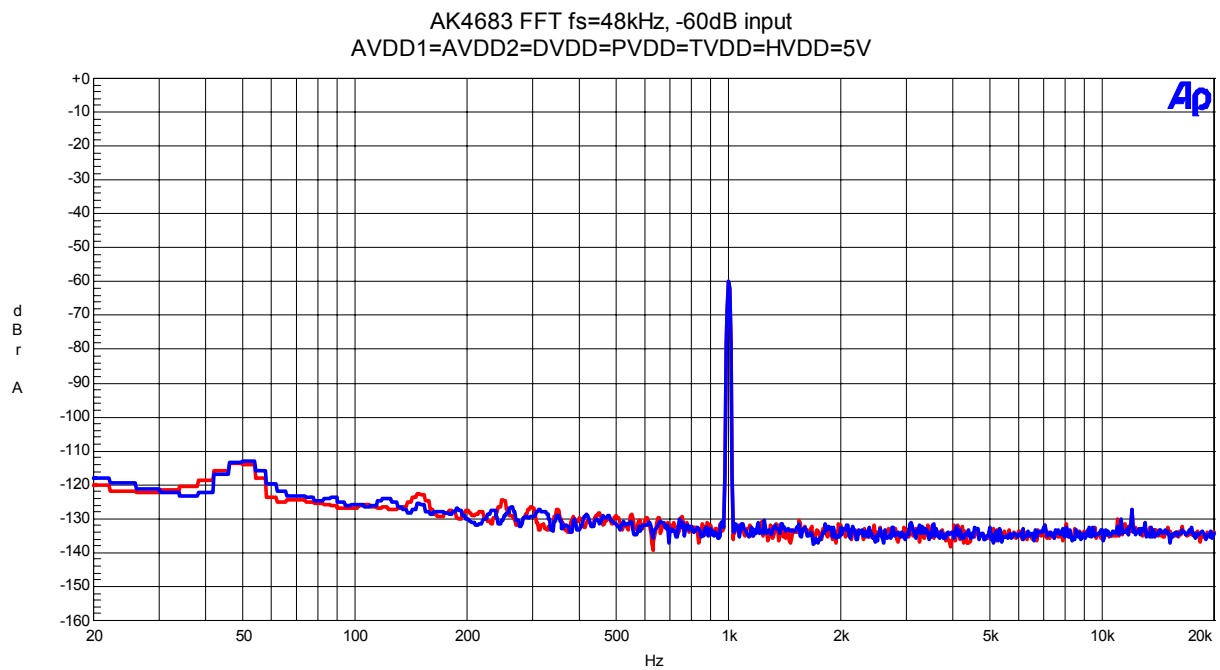
Figure 27. FFT(Input Frequency =1kHz, Input Level=-60dBFS)
