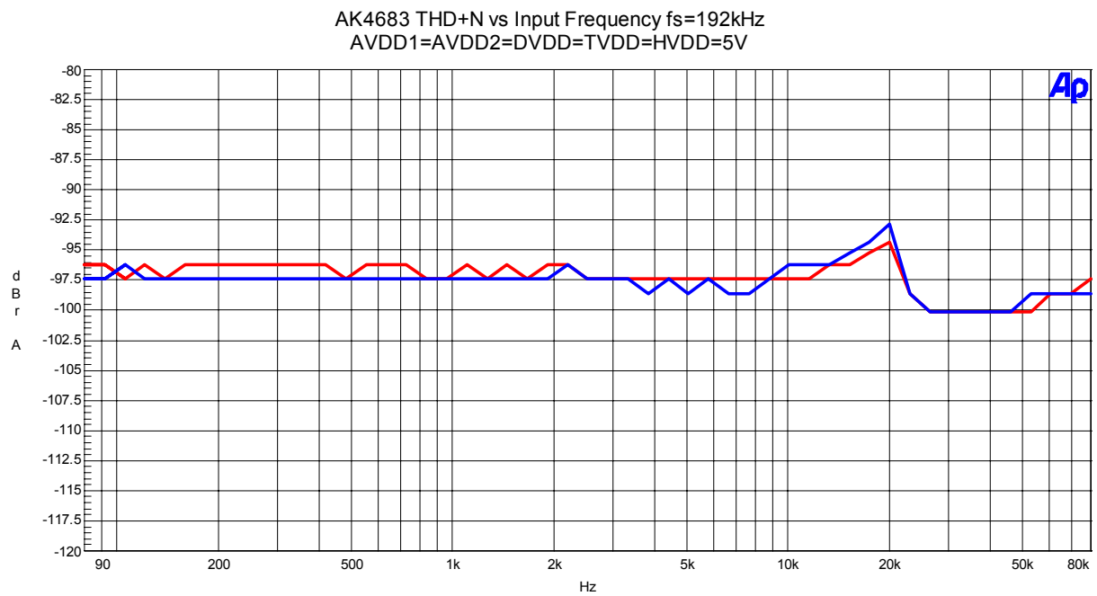
Figure 49. THD+N vs Input Frequency (Input Level=0dBFS)
