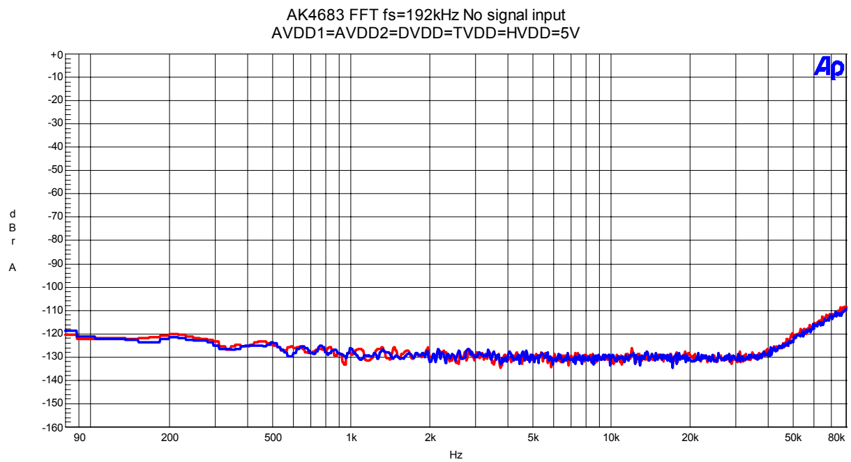
Figure 47. FFT(noise floor)
