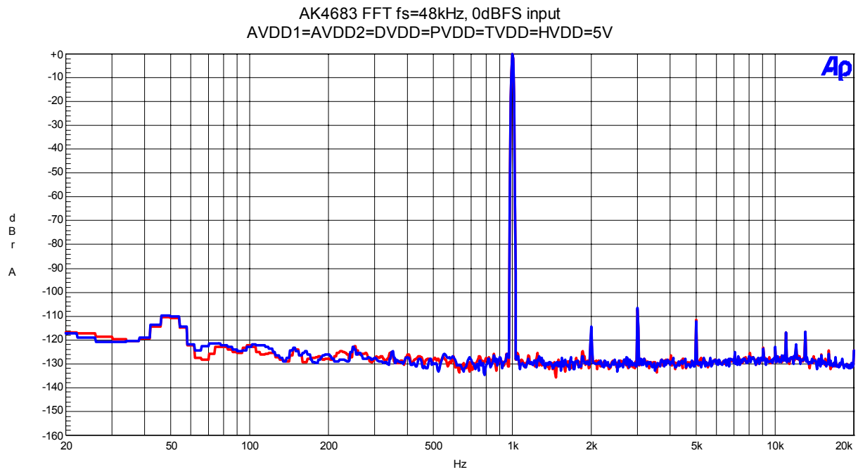
Figure 26. FFT(Input Frequency =1kHz, Input Level=0dBFS)
