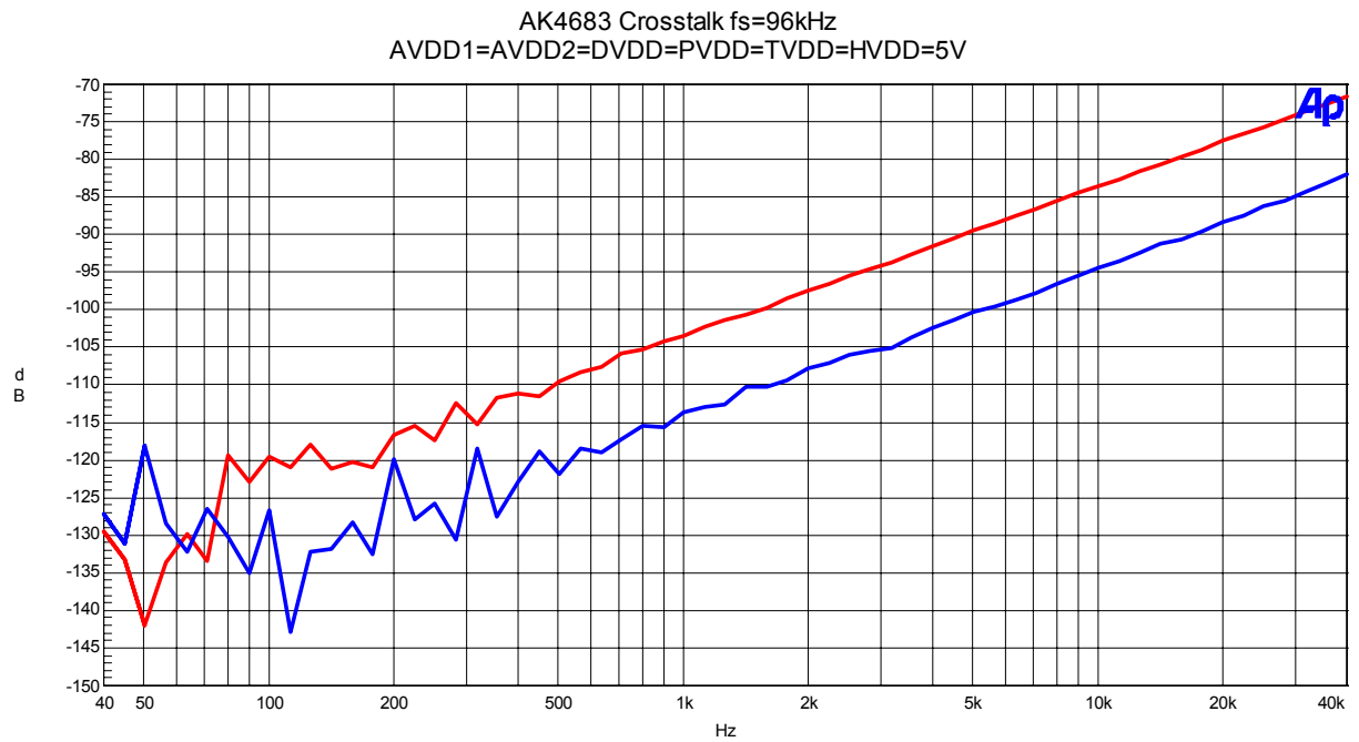
Figure 25. Crosstalk (Input Level=-0.5dBFS)
