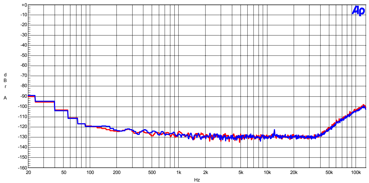
Figure 29. FFT(out-of-band noise)
