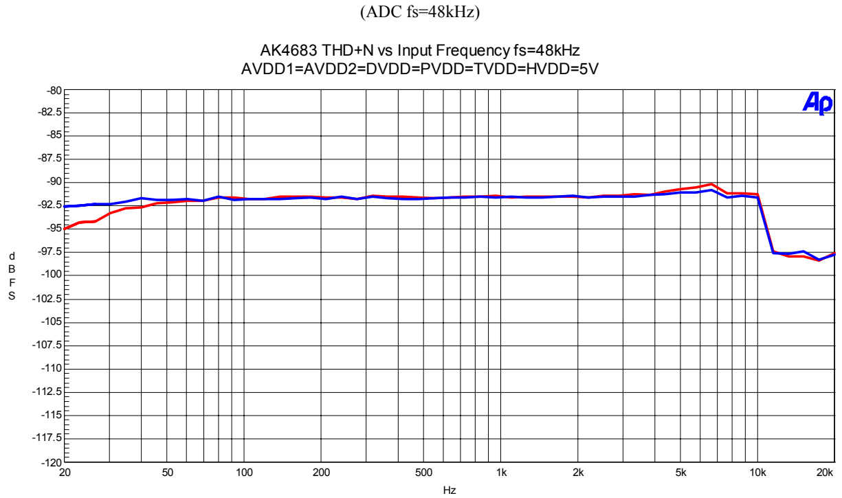
Figure 14. THD + N vs Input Frequency (Input Level=-0.5dBFS)
