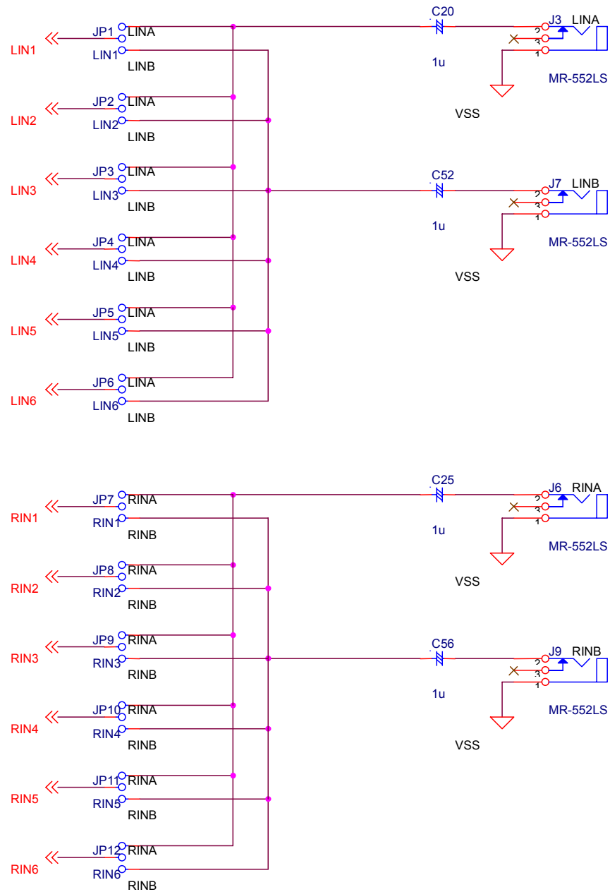
Figure 3. Analog Input Circuit
