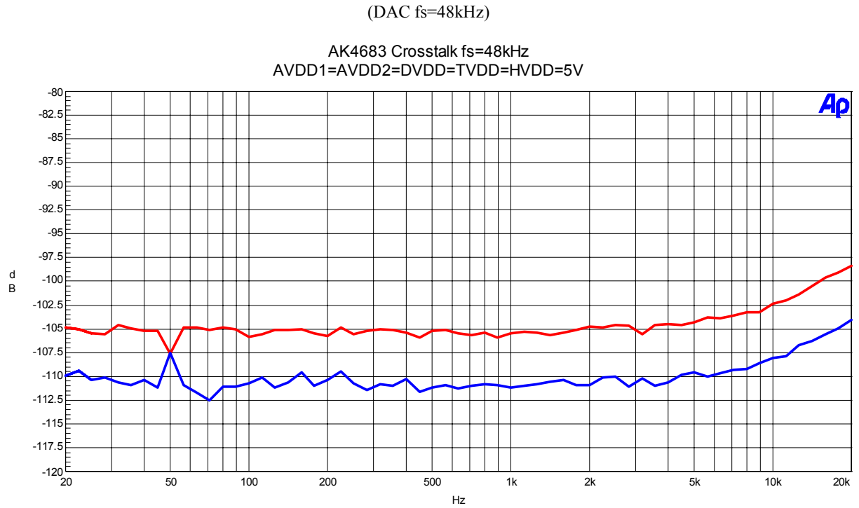
Figure 34. Cross-talk (Input Level=0dBFS)
