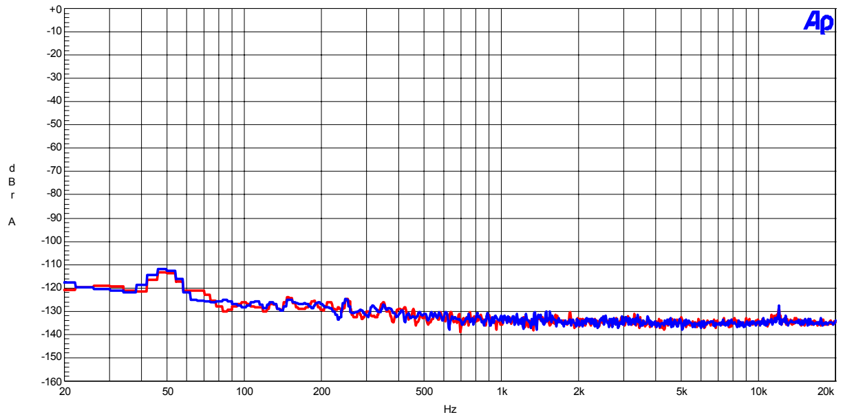
Figure 28. FFT(noise floor)
