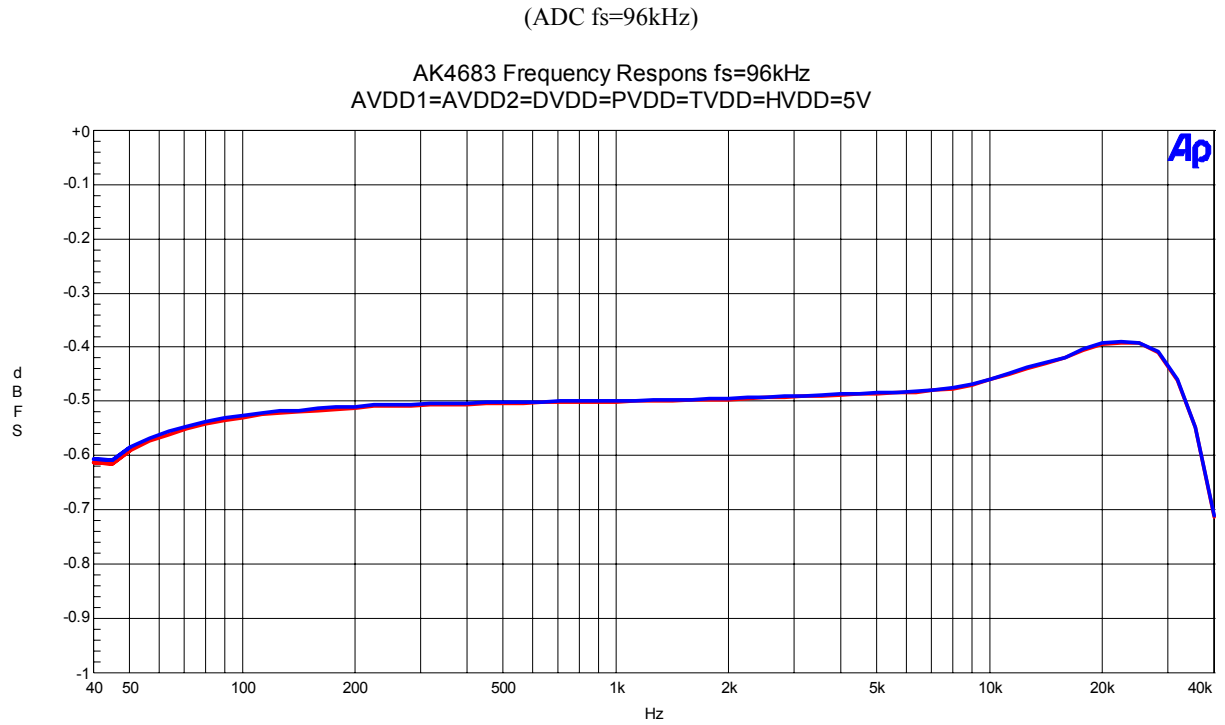
Figure 24. Frequency Response (Input Level=-0.5dBFS)
