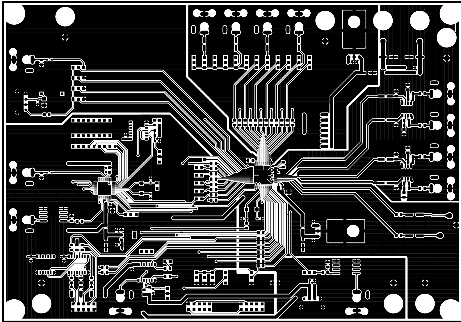
AKD4683-B L1
