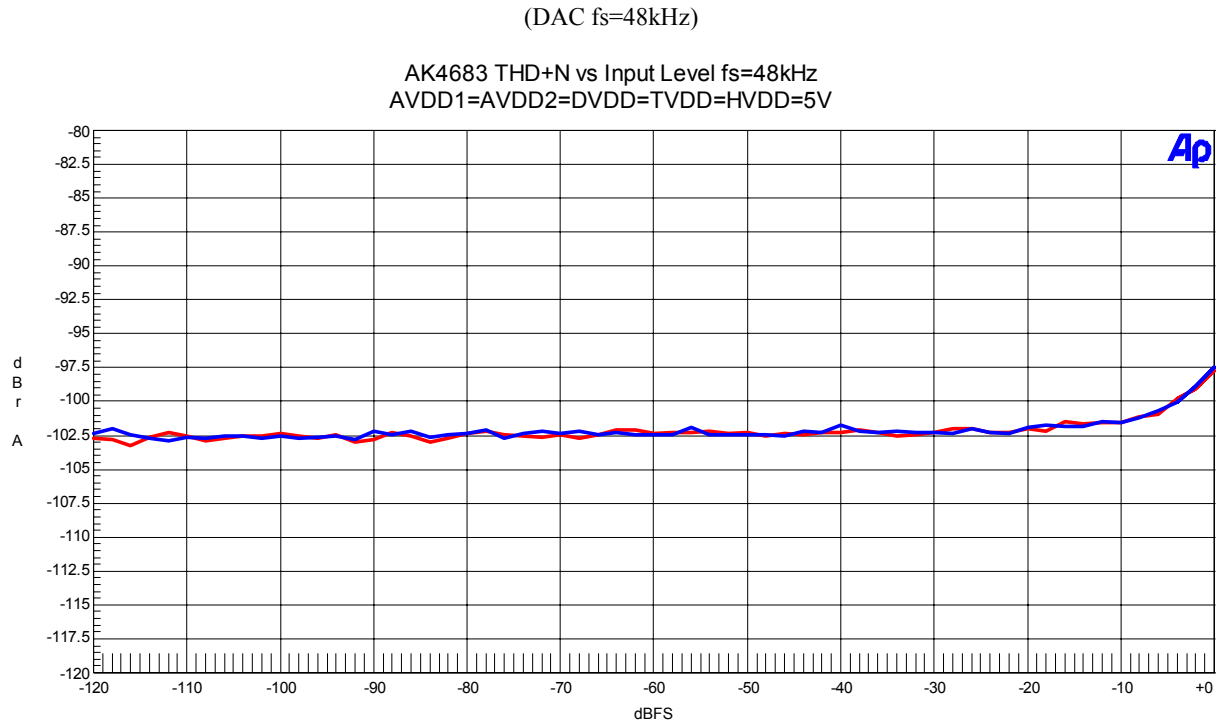
Figure 30. THD+N vs Input Level (Input Frequency =1kHz)
