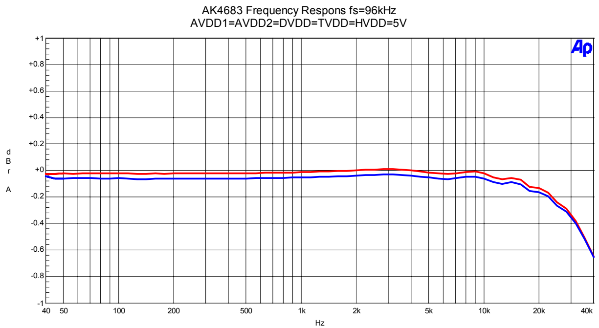
Figure 42. Frequency Response (Input Level=0dBFS)
