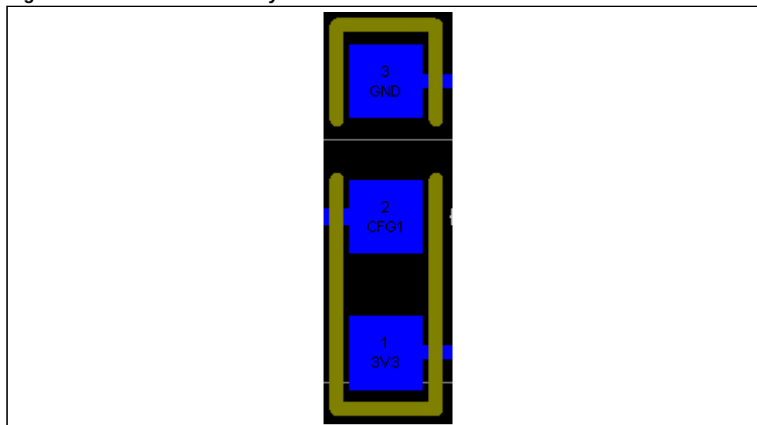
Figure 9. Resistor assembly
