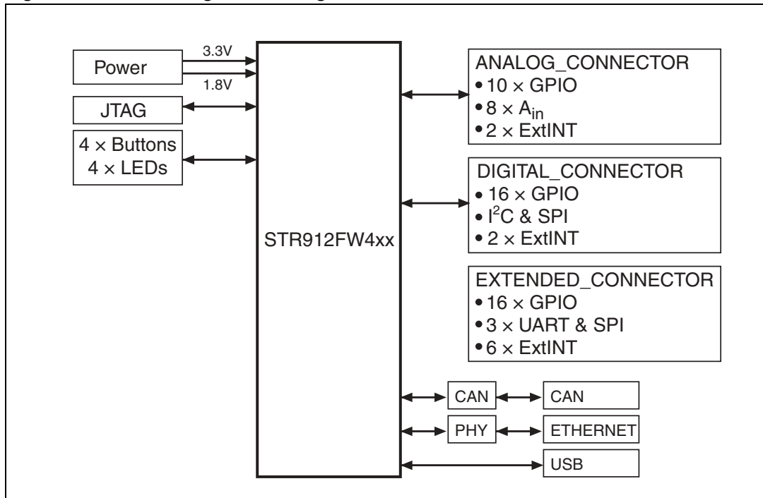
Figure 2. STR9 Dongle block diagram
