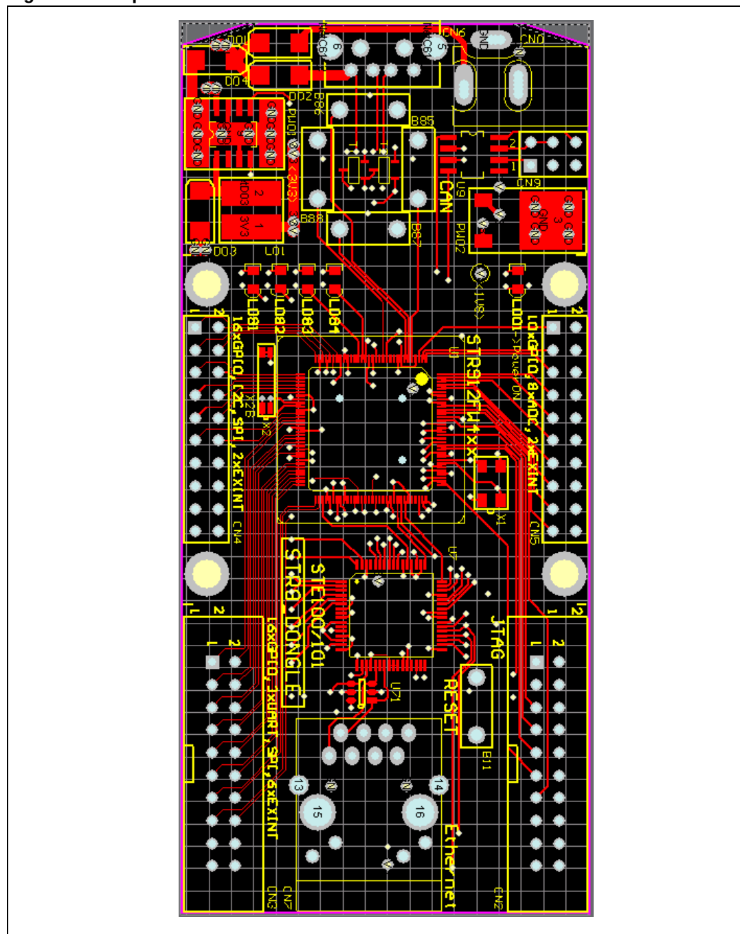
Figure 7. Top view
