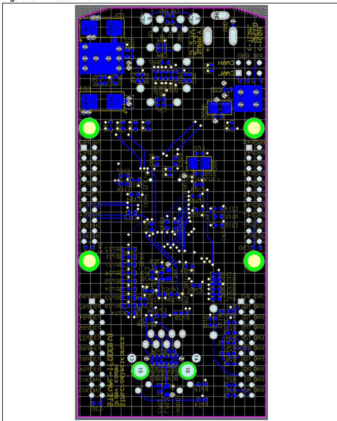
Figure 8. Bottom view
