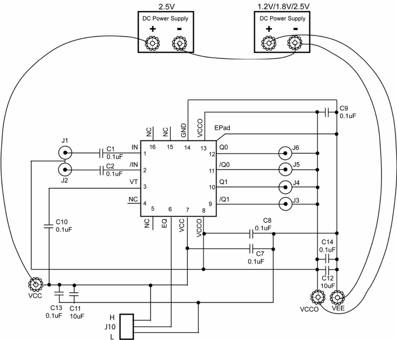
SY56011R AC-Coupled Evaluation Board
