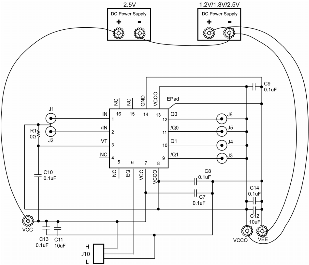
SY56011R DC-Coupled Evaluation Board
