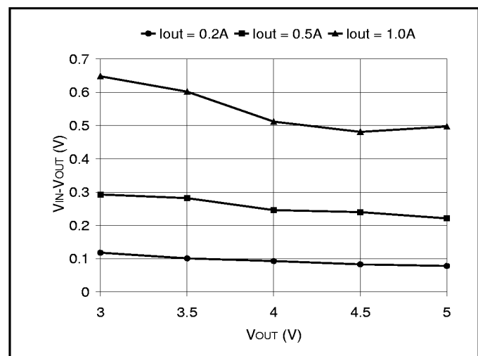
Figure 3. Typical dropout voltage vs. I_{OUT} and V_{OUT} .
