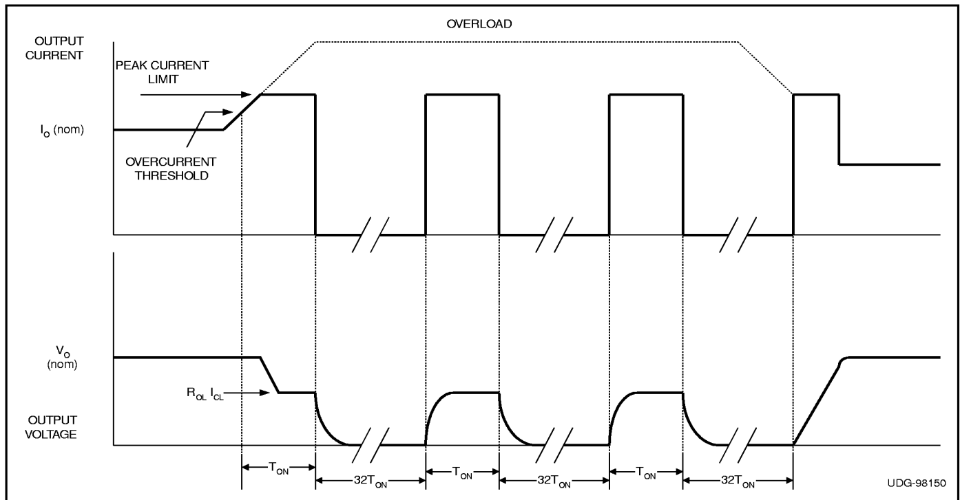
Figure 1. UCC381 short circuit timing.
