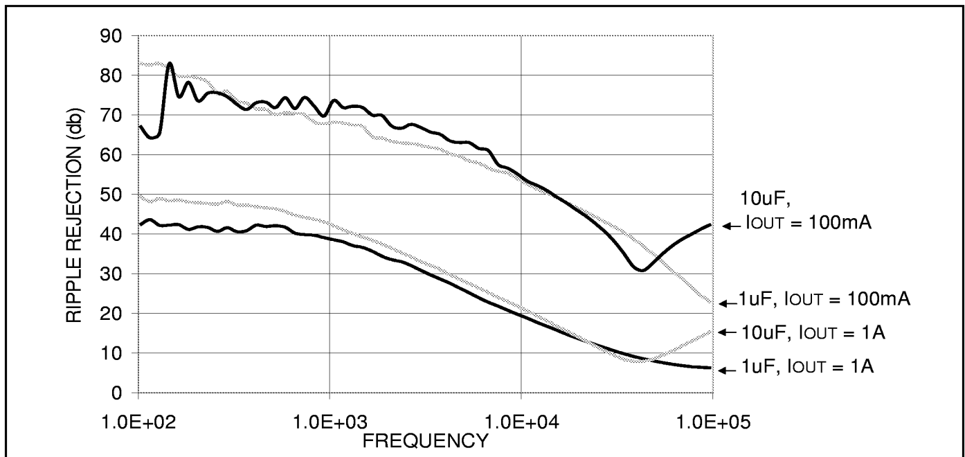
Figure 5. Ripple rejection vs. frequency.
