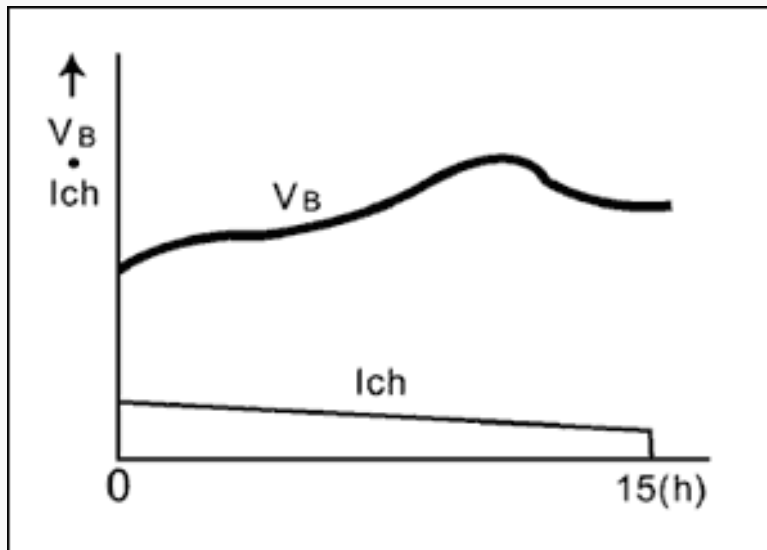
Figure 1. Semi-constant current charging, chiefly used in applications like shavers, digital cordless phones, and toys.
