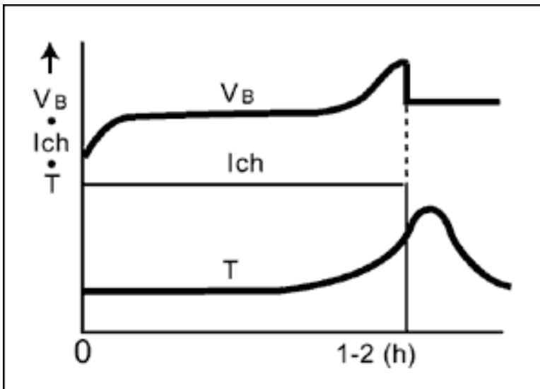
Figure 4. Charging is terminated through -dT/dt cutoff in applications like power tools and electric tools.
