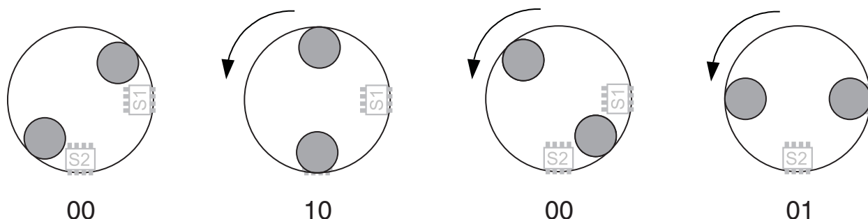
Figure 6. Sensor/Magnet Configurations Resulting in S2/S1 Values
