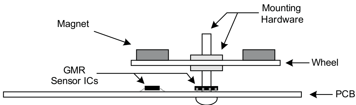
Figure 3. Wheel Apparatus
