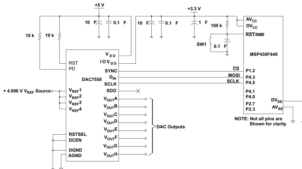
Figure 3. MSP430F449 and DAC7558 Circuit Diagram
