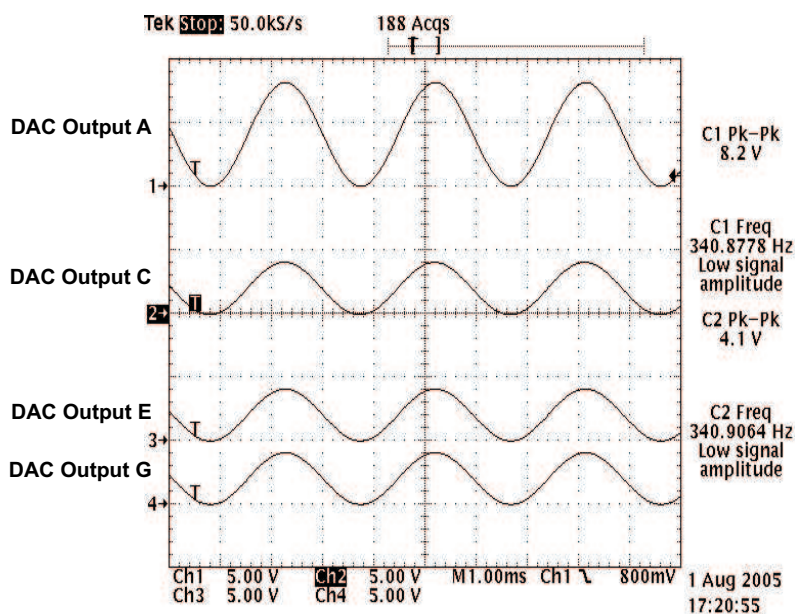
Figure 6. DAC Output Waveform Diagram
