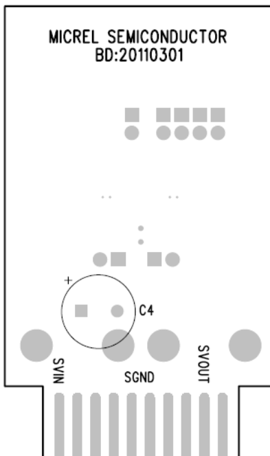
MIC5282YMME Evaluation Board – Bottom Silkscreen
