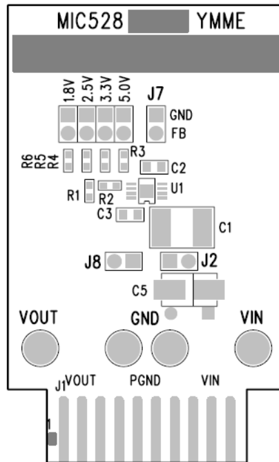
MIC5282YMME Evaluation Board – Top Silkscreen Layer
