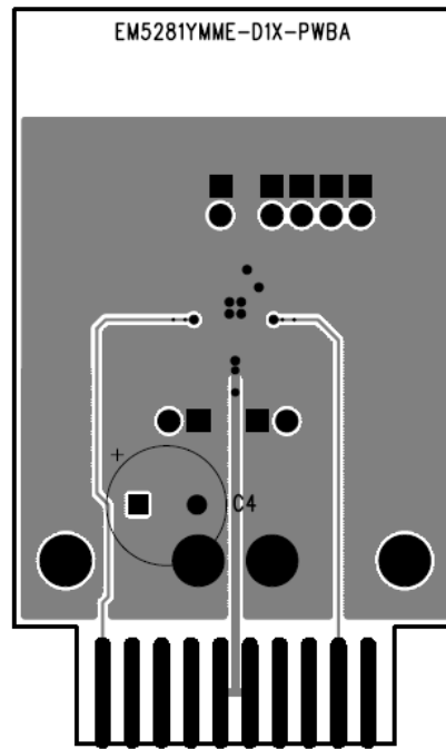
MIC5282YMME Evaluation Board – Bottom Layer
