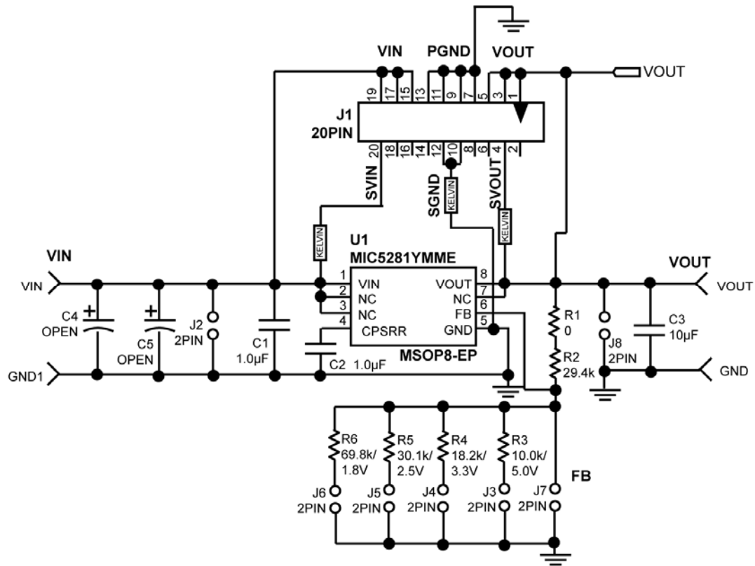
MIC5282YMME Evaluation Board (J1 is for test purposes only)
