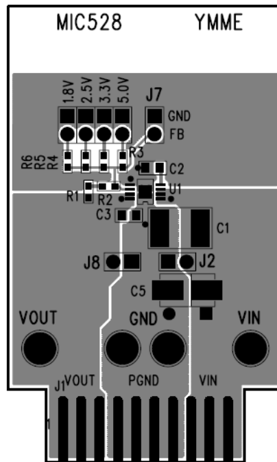
MIC5282YMME Evaluation Board – Top Layer
