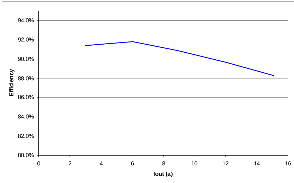
15 Amp Output
