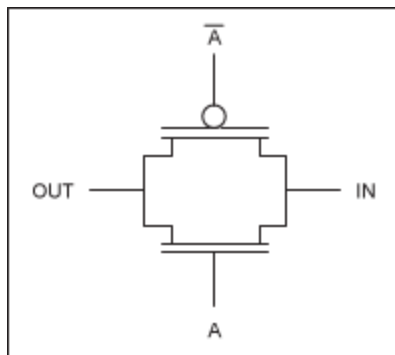
Figure 1. Schematic representation of a transmission gate.
