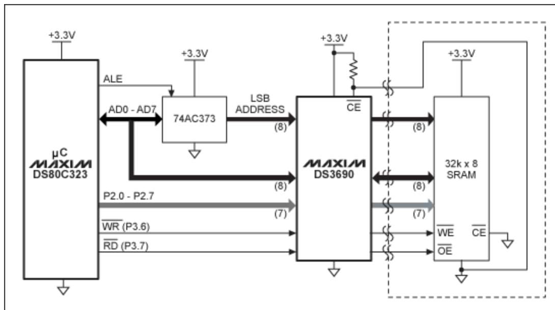
Figure 3. Typical DS3690 application circuit.
