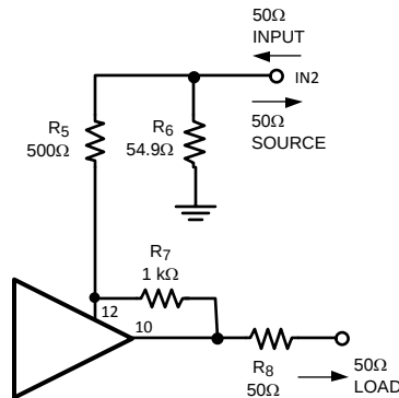
Figure 3. Summing a High-Speed Signal Into The Output
