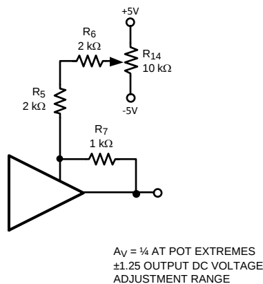
Figure 4. Summing in an Output DC Offset
