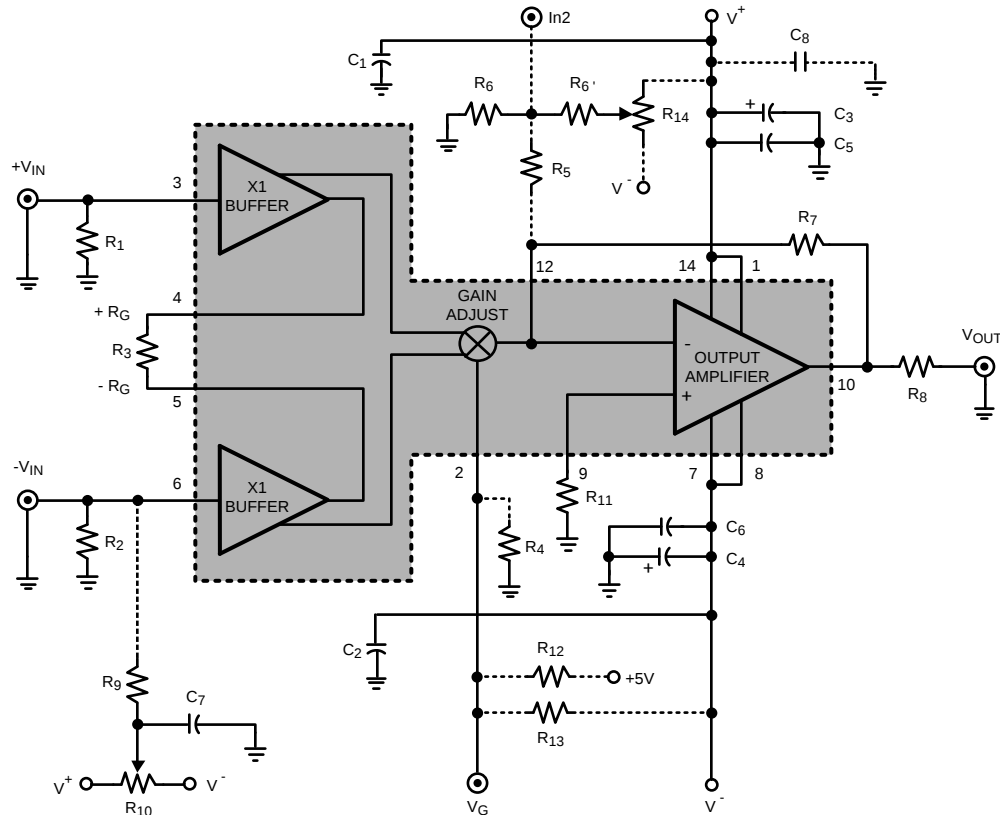
Figure 1. External Components & Amplifier Internal Block Diagram
