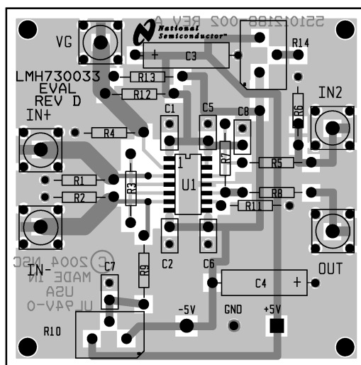
Figure 6. LMH730033 (Component and Circuit Side)
