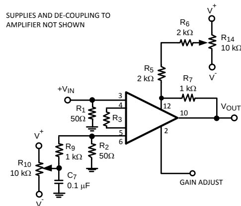
Figure 5. Input and Output Stage DC Nulling
