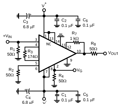
Figure 2. Basic Connection
