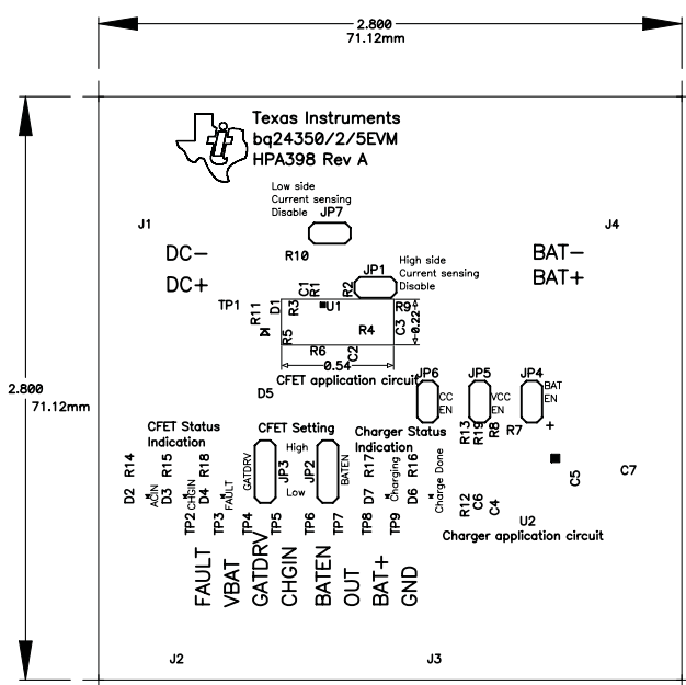
Figure 4. Top Silk Screen
