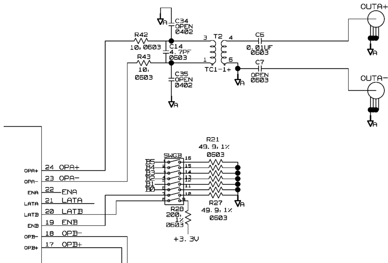
Figure 2. Output Schematic
