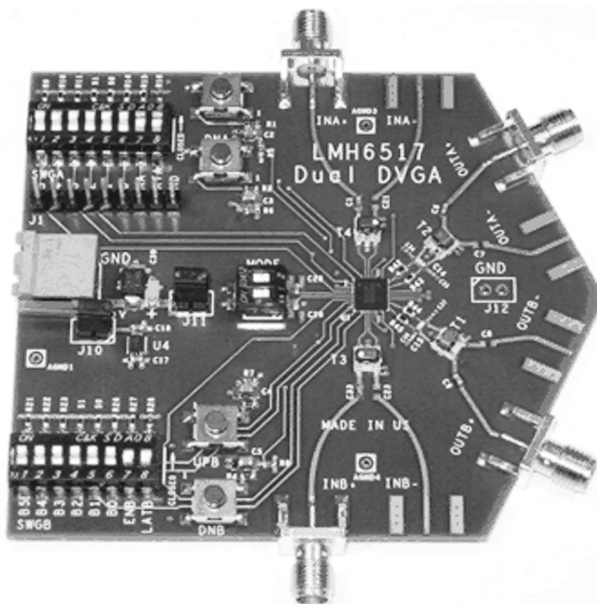
Figure 1. LMH6517EVAL-R1 Evaluation Board
