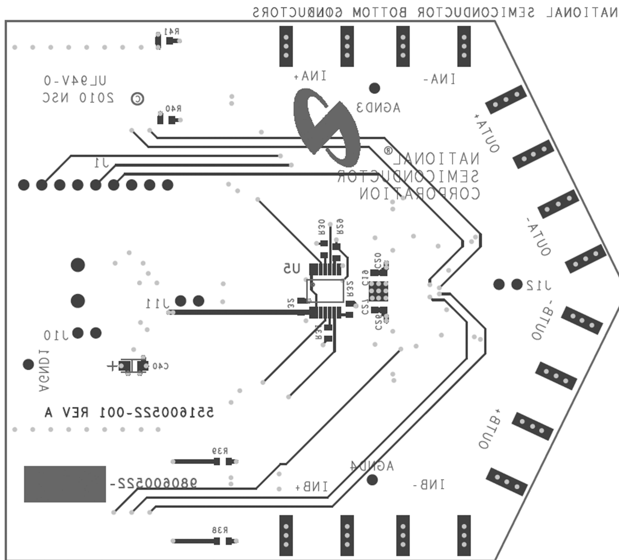
Figure 5. Evaluation Board Bottom Layer
