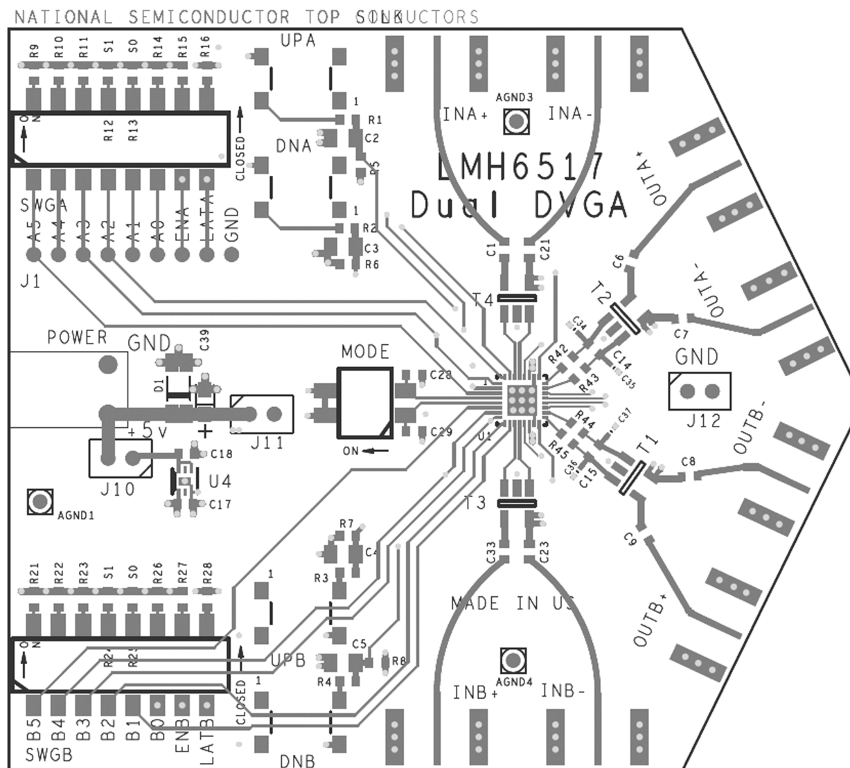
Figure 4. Evaluation Board Top Layer
