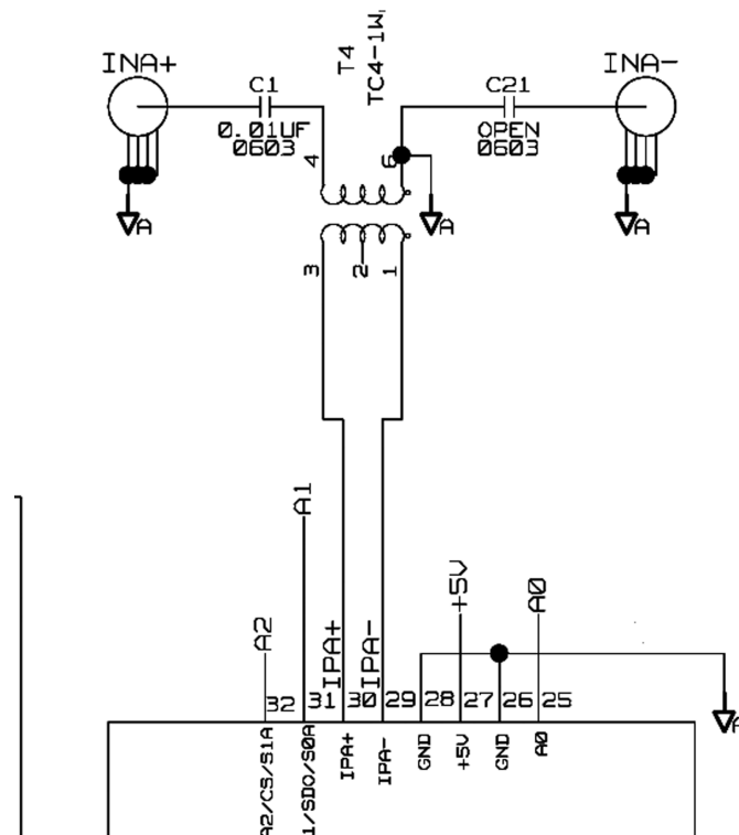
Figure 3. Input Schematic
