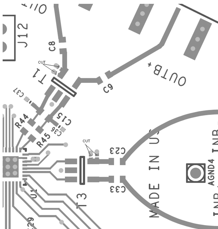
Figure 7. Trace Cuts for Differential Input and Output
