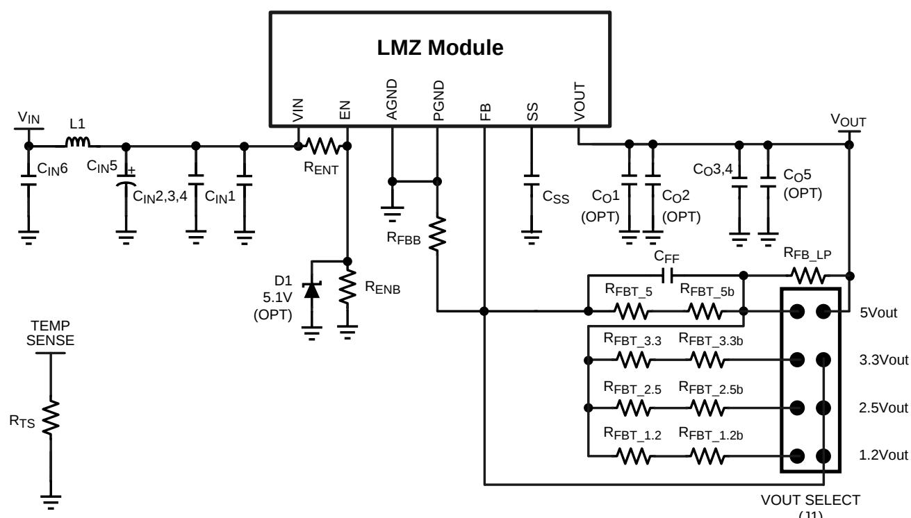
Figure 1. Simplified Schematic
