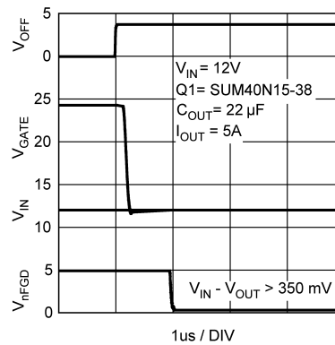
Figure 3. MOSFET Test, No Fault
