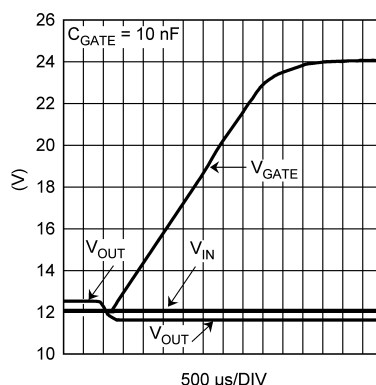
Figure 1. Forward Waveforms
