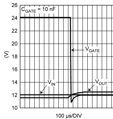
Figure 2. Reverse Waveforms
