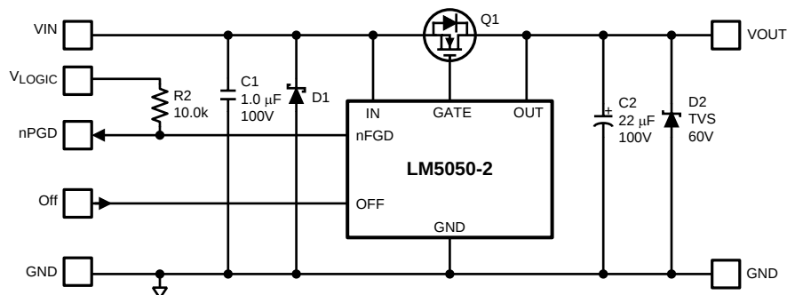
Figure 5. Schematic Diagram
