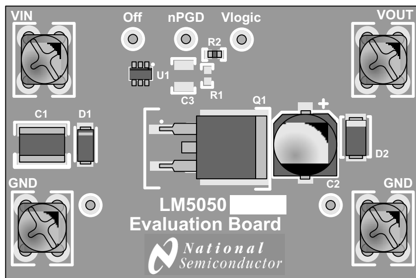
Figure 6. Component Placement
