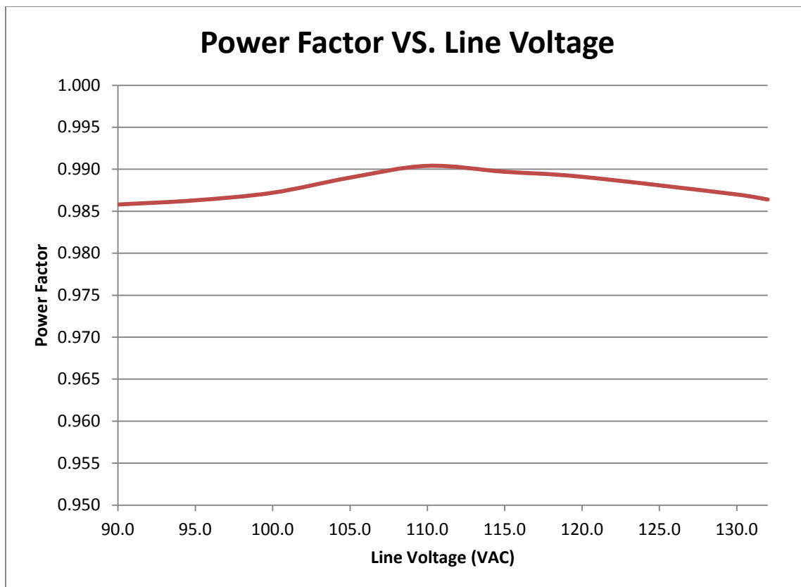
FIGURE 3. Power Factor vs. Line Voltage from 90VAC to 132VAC/60Hz
