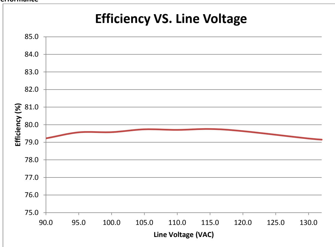
FIGURE 1. Efficiency vs. Line Voltage from 90VAC to 132VAC/60Hz
