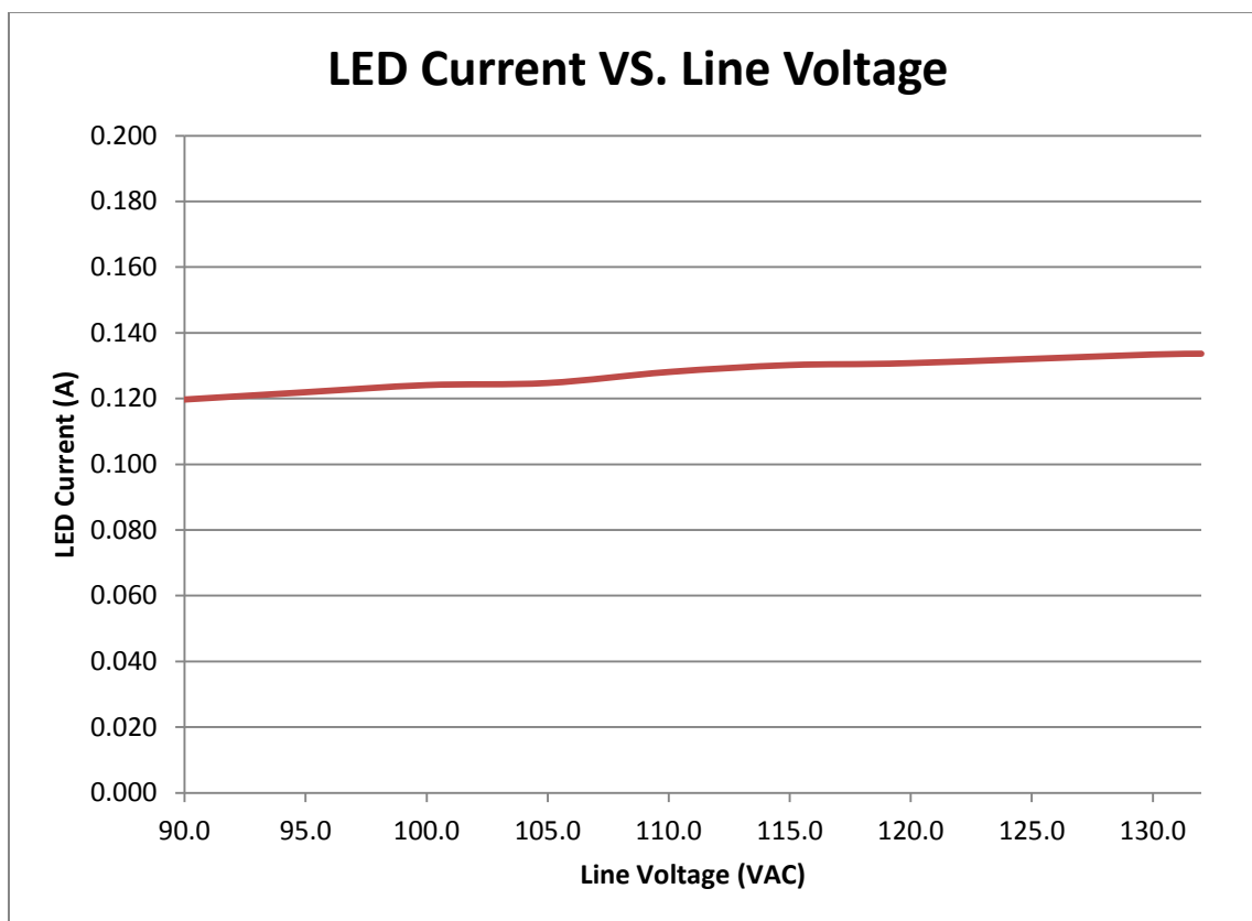
FIGURE 2. LED Current vs. Line Voltage from 90VAC to 132VAC/60Hz
