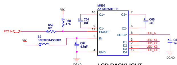
LCD BACKLIGHT
