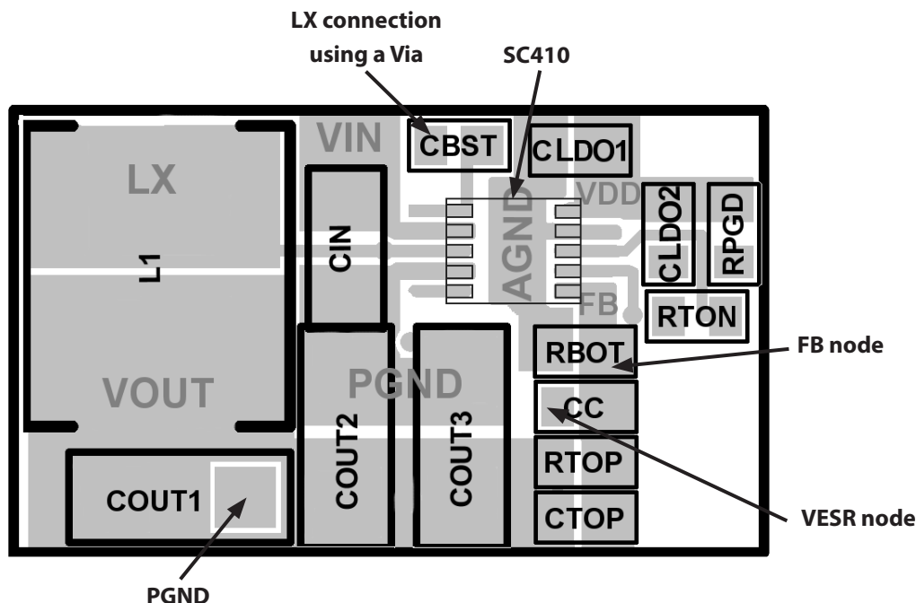
Figure 11 — PCB Layout
