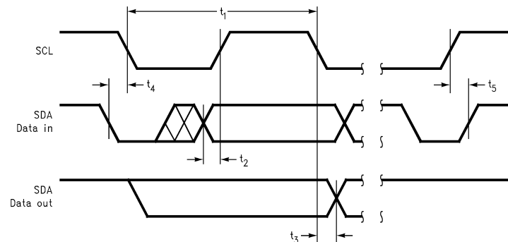
Figure 69. I²C Timing Diagram
