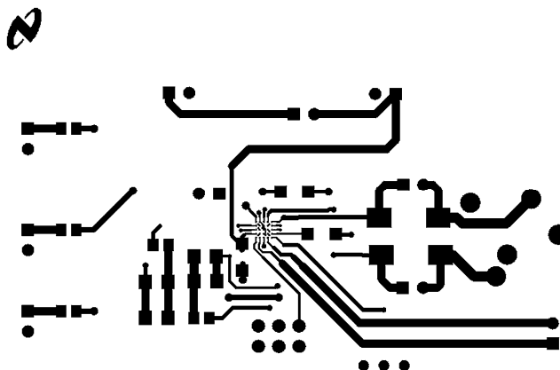
Figure 74. Top Layer
