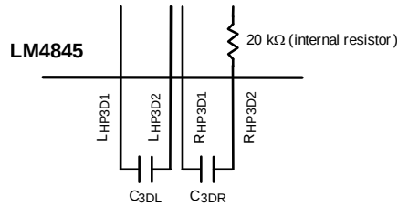
Figure 71. External 3D Effect Capacitors
