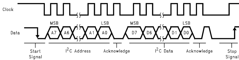
Figure 68. I²C Bus Format
