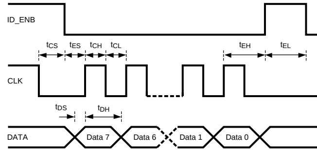
Figure 70. SPI Timing Diagram
