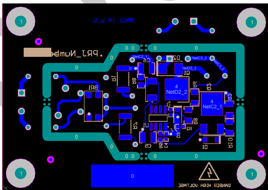
Figure 11: Bottom Layer and Bottom Overlay (Bottom view)
