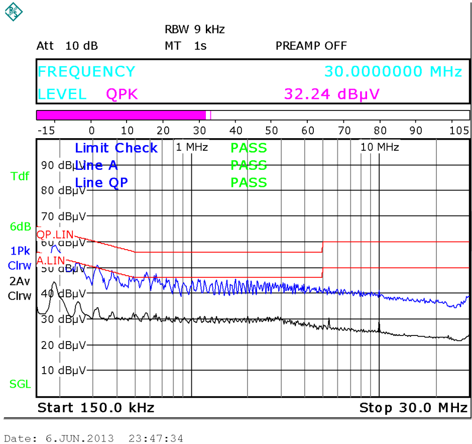
Figure 8: 230VAC Line-Conducted EMI Scan
