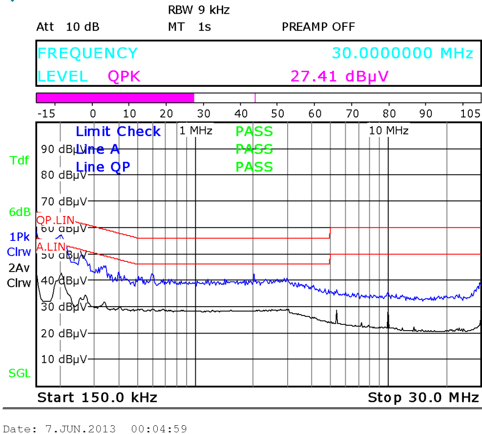
Figure 9: 230VAC Neutral-Conducted EMI Scan
