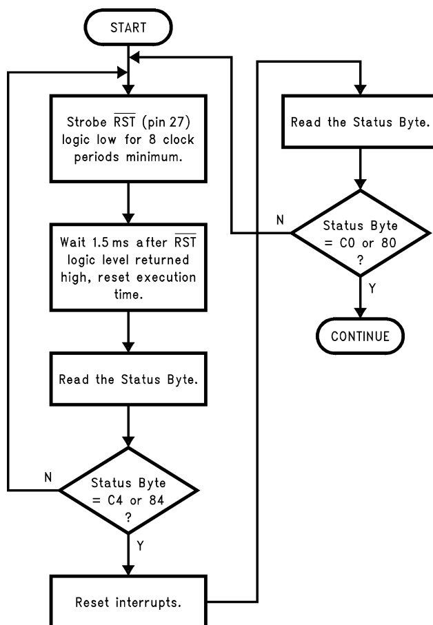
Figure 4. Hardware Reset Block
