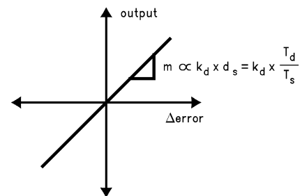
Figure 22. Derivative Term
