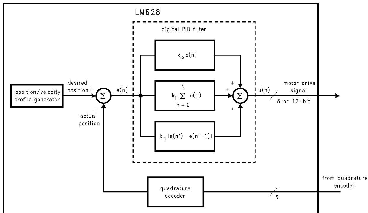
Figure 8. LM628—Simplified Block Diagram Form
