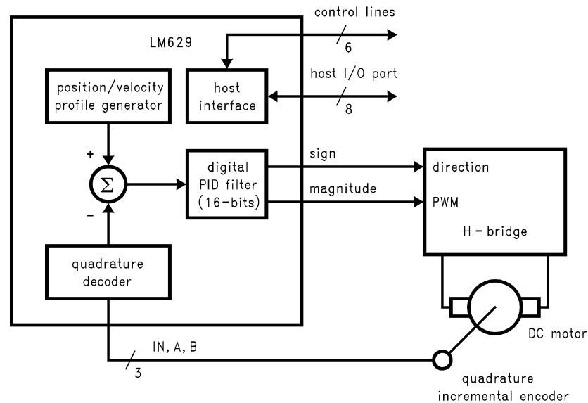
Figure 2. LM629-Based Motor Control System
