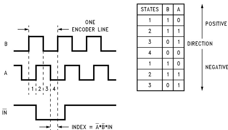
Figure 13. 3-Channel Quadrature Encoder Signals
