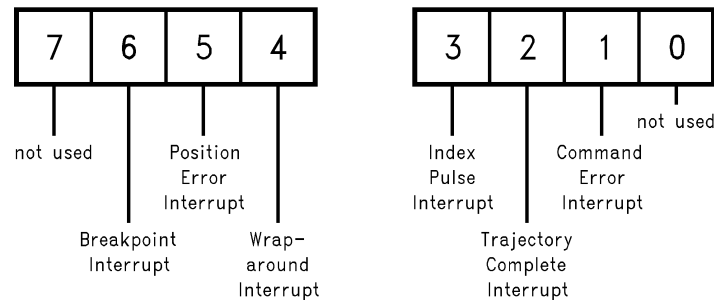
Figure 7. Low Byte — Interrupt Mask/Reset Bit Allocations
