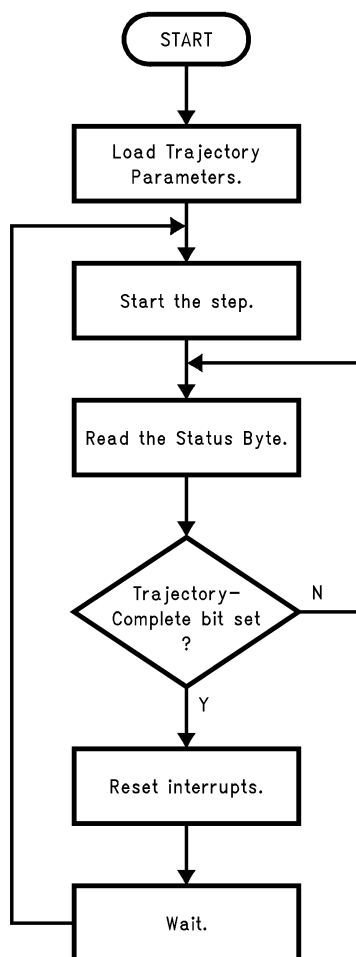
Figure 23. Step Generation Section of Filter Tuning Program
