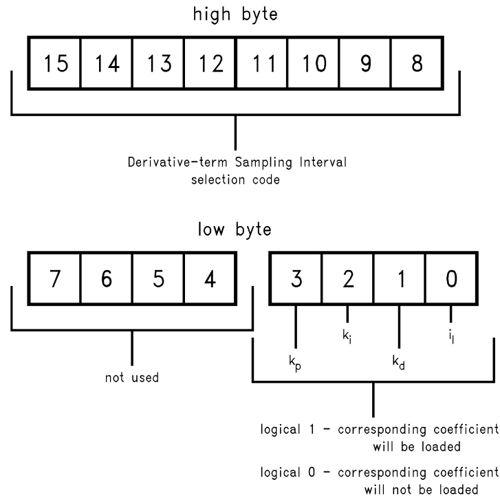
Figure 9. Filter Control Word Bit Allocation
