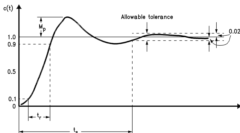
Figure 18. Unit Step Response Curve Showing Transient Response Attributes
