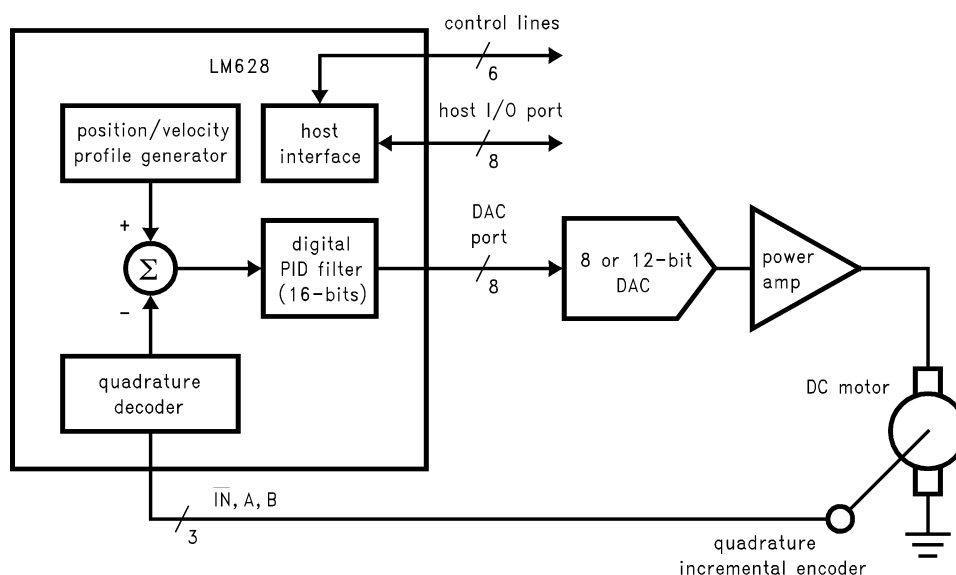
Figure 1. LM628-Based Motor Control System
