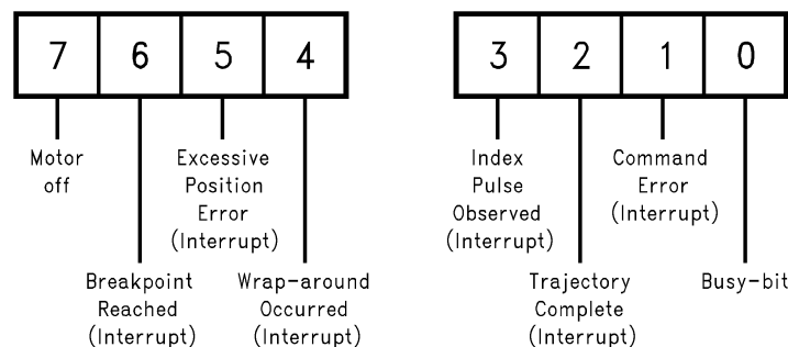
Figure 5. Status Byte Bit Allocation
