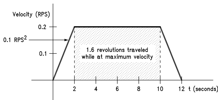
Figure 12. Velocity Profile for Simple Absolute Position Move Program
