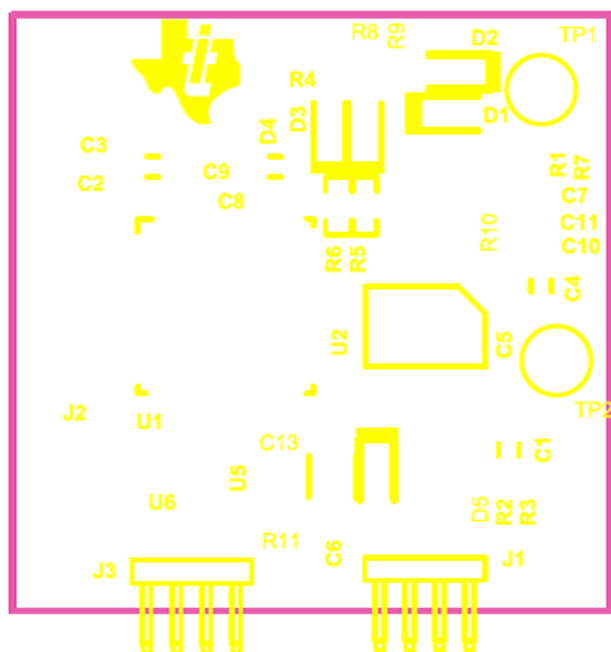
Figure 78. Top Overlay
