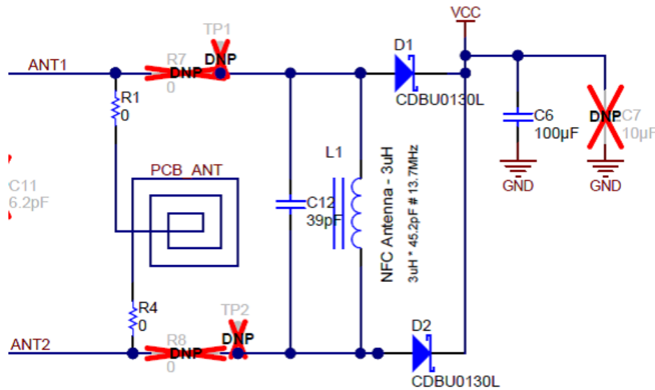
Figure 11. Split Power and RF Antenna
