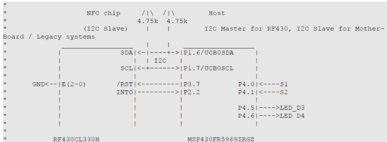
Figure 27. Overview of the Hardware Corresponding to TIDA-00230 Configuration
