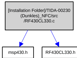
Figure 49. RF430CL330.c Dependency Graph
