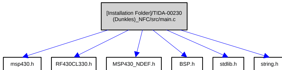
Figure 43. main.c Dependency Graph
