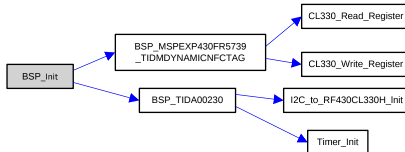
Figure 22. BSP_Init Call Graph
