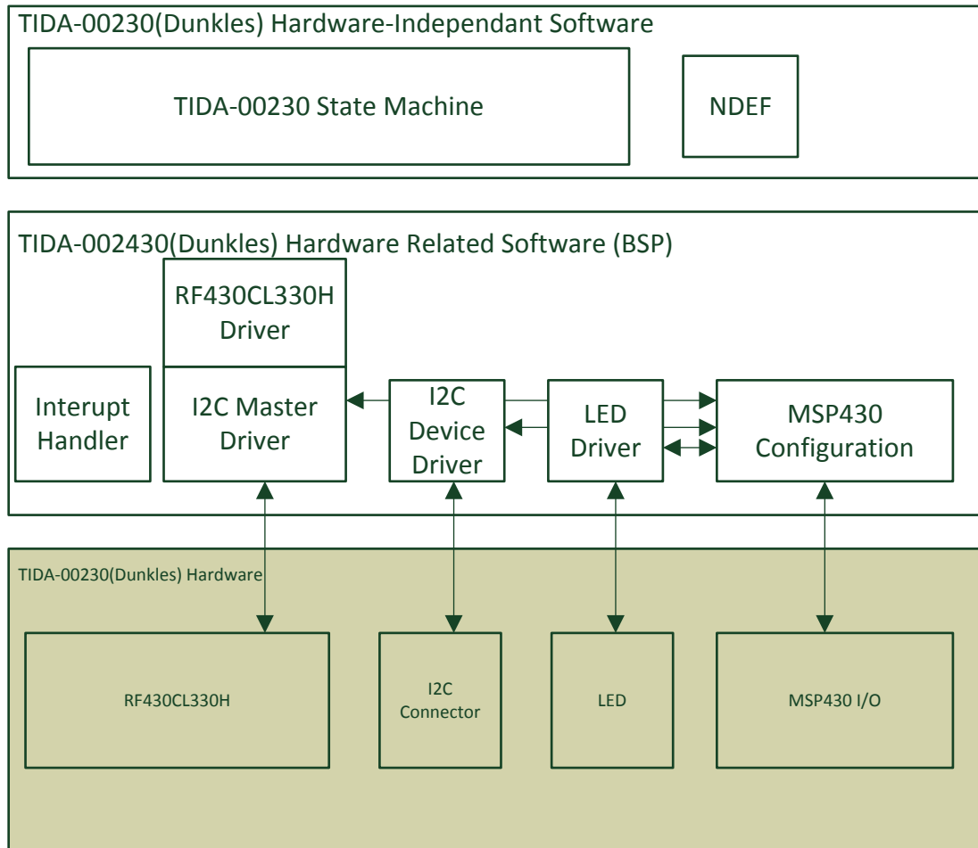
Figure 3. Software Block Diagram
