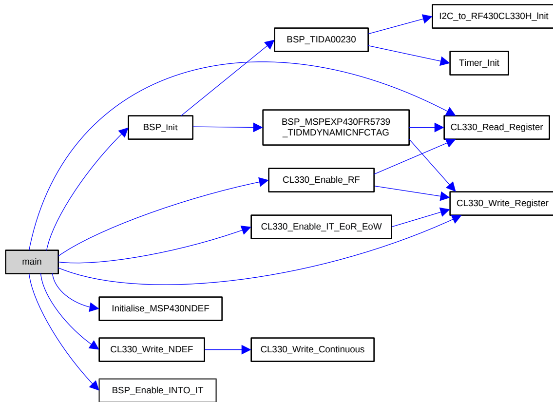
Figure 44. main Call Graph
