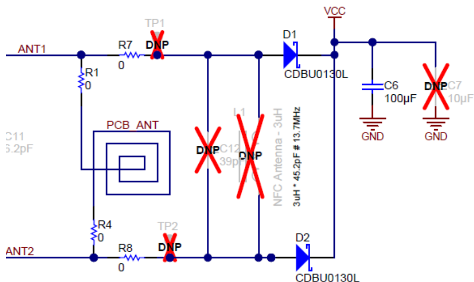
Figure 9. PCB Antenna (Default Variant)
