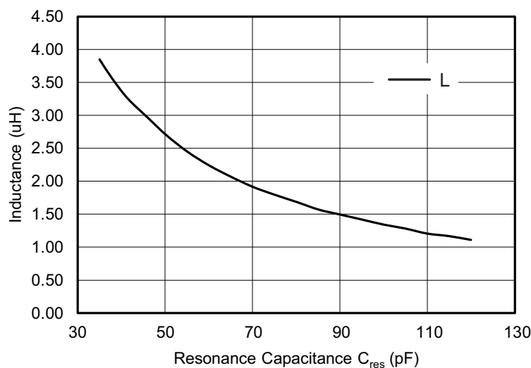
Figure 71. L versus C_{res} at f_{res} = 13.7 MHz
