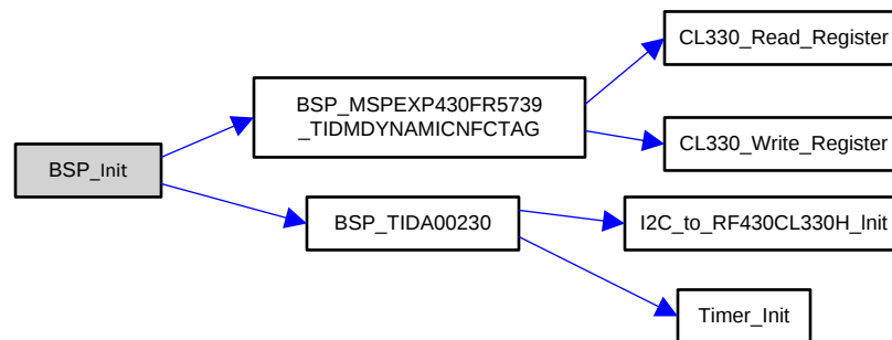
Figure 34. BSP_Init Call Graph
