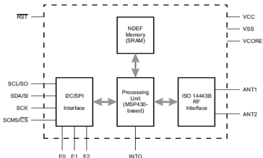
Figure 13. RF430CL330H Functional Block Diagram
