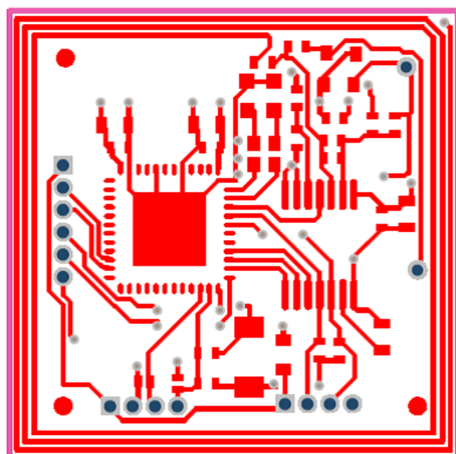
Figure 80. Top Layer
