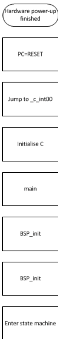
Figure 12. Software Power-Up Sequence
