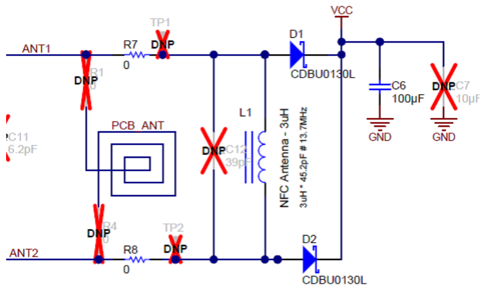
Figure 10. Ferrite NFC Antenna
