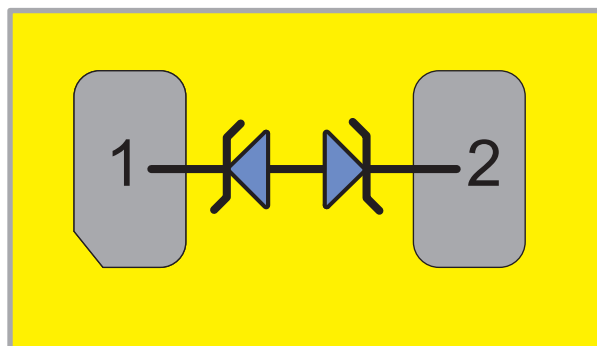
Figure 15. TPD1E10B06DPYR Functional View
