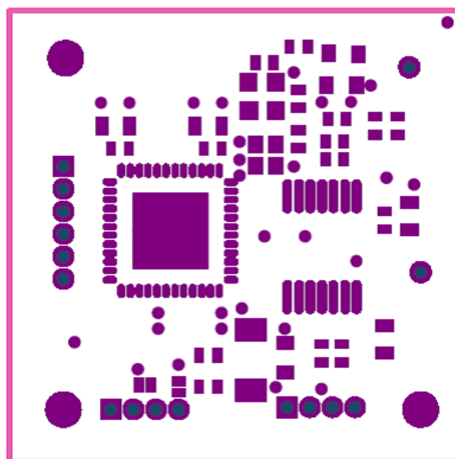
Figure 79. Top Solder Mask
