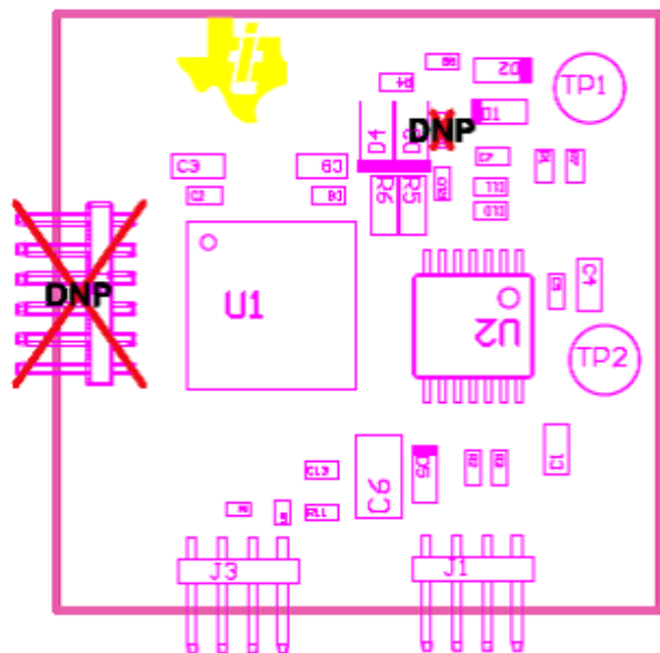
Figure 82. Assembly Drawing: Top
