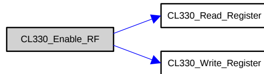
Figure 52. CL330_Enable_RF Call Graph
