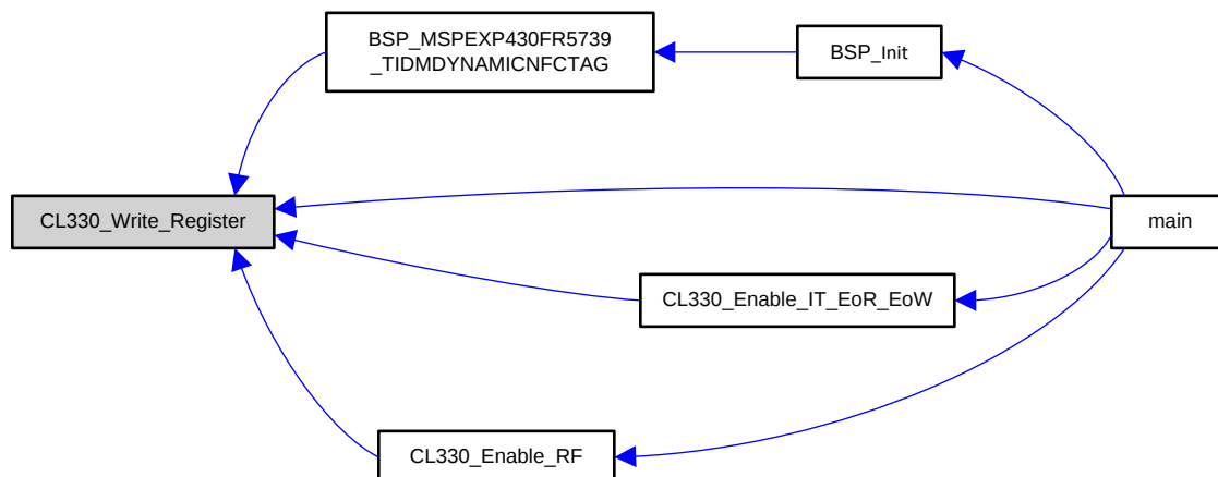
Figure 58. CL330_Write_Register Caller Graph
