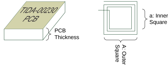
Figure 4. Dimensions for Calculating Antenna Inductance
