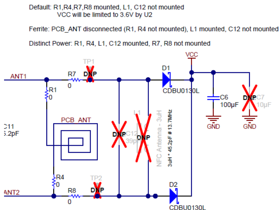
Figure 7. Antenna Schematics Variants, Extracted from Main Schematics (Default Variant)
