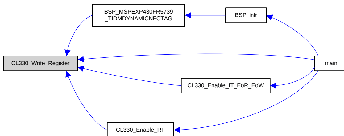
Figure 68. CL330_Write_Register Caller Graph
