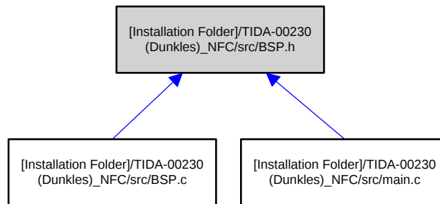
Figure 32. BSP.h Dependency Graph
