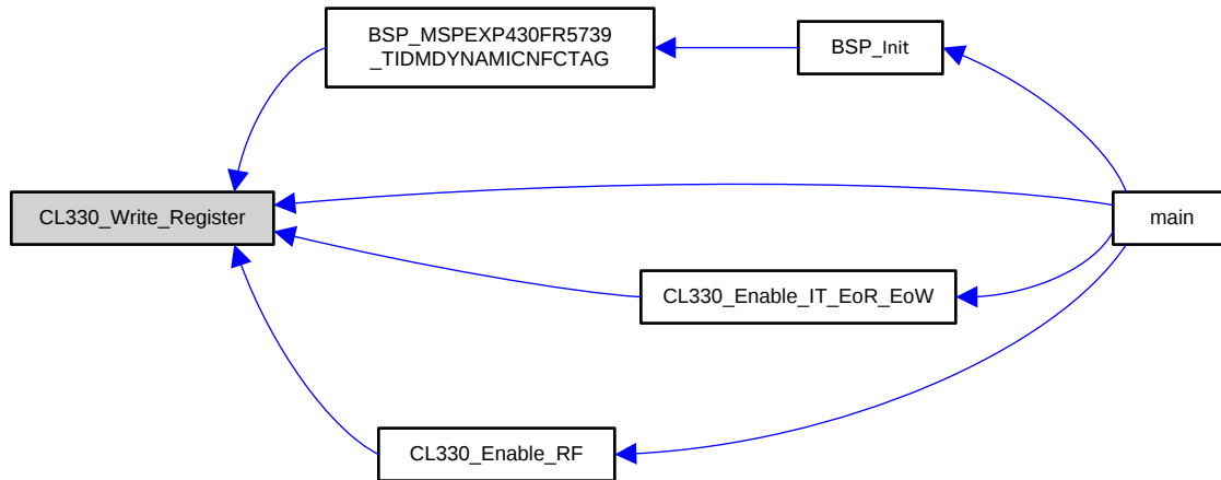
Figure 64. CL330_Write_Register Caller Graph
