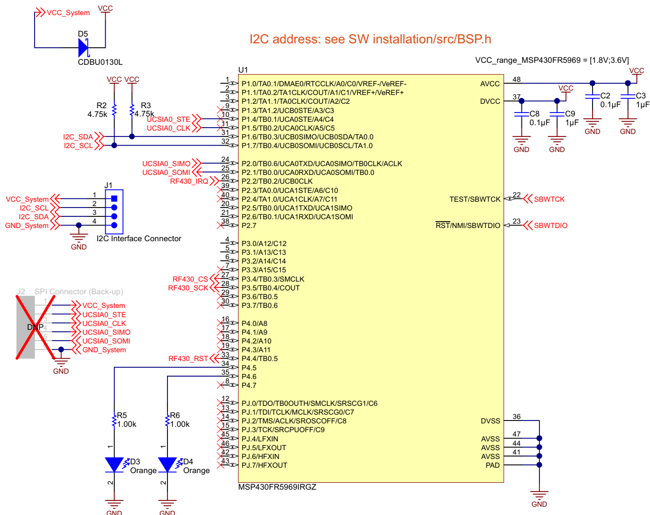
Figure 75. MSP430 Microcontroller
