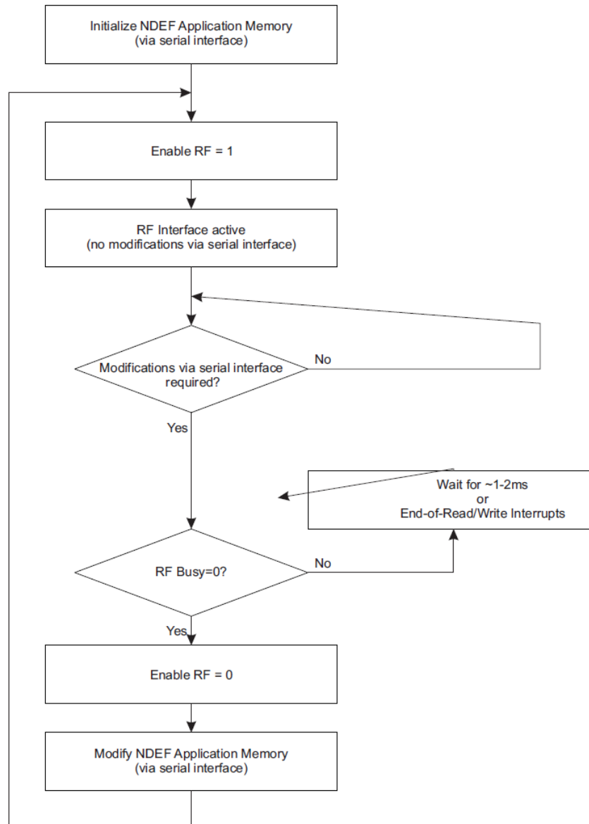
Figure 19. Recommended NDEF Data Memory Flow
