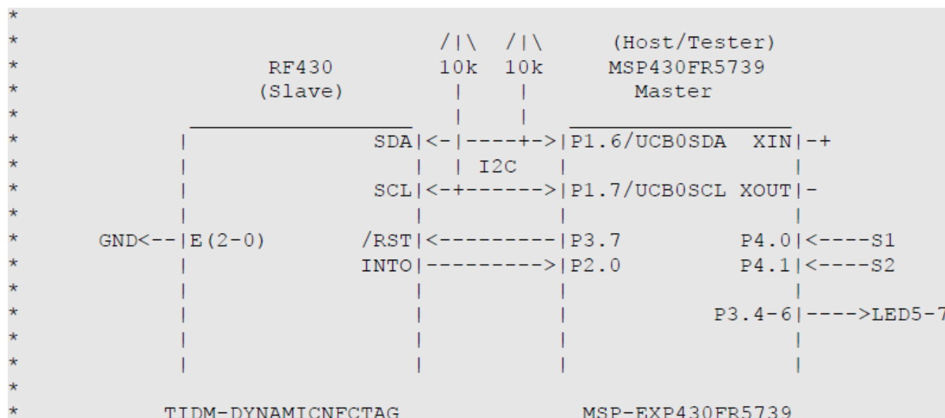
Figure 36. Overview of Hardware Configuration for Software Configuration MSPEXP430FR5739_TIDMDYNAMICNFCTAG
