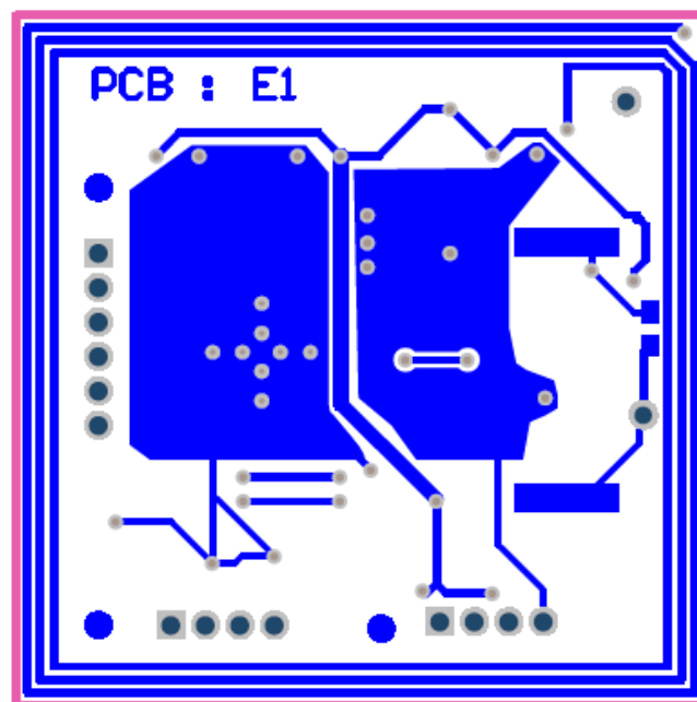
Figure 81. Bottom Layer
