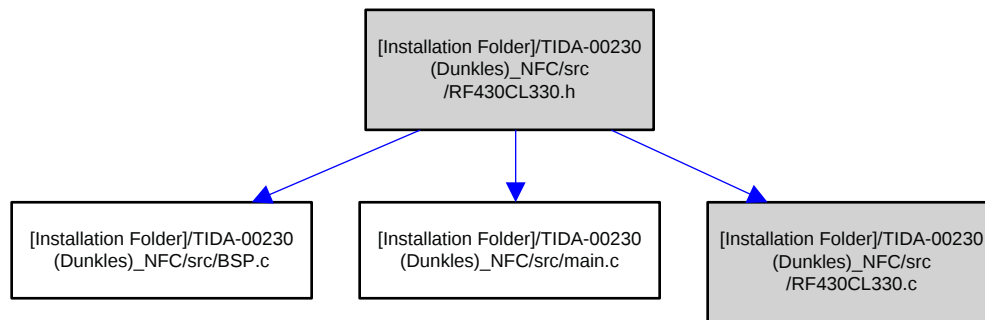
Figure 59. RF430CL330.h Dependency Graph
