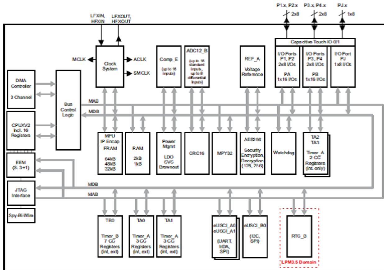
Figure 14. MSP430FR5969 Functional Block Diagram
