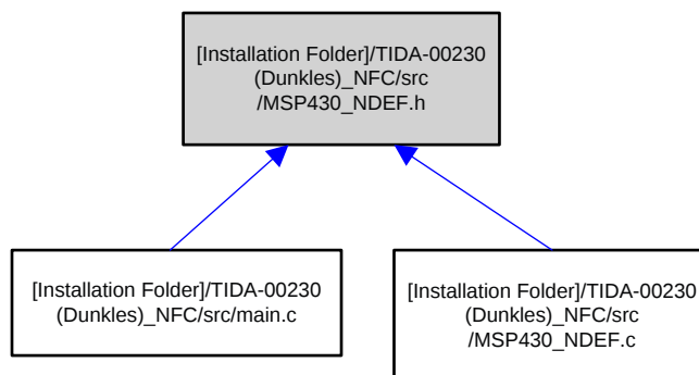
Figure 47. MSP430_NDEF.h Dependency Graph
