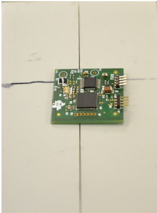
Figure 69. Top View of PCB Antenna Design on Reference Antenna
