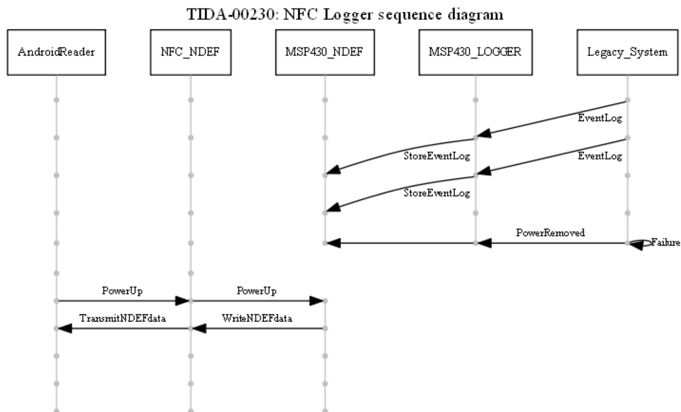
Figure 18. Sequence Diagram
