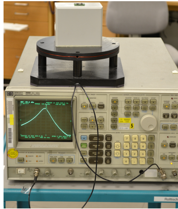
Figure 70. Front View of Design on Test Antenna Connected to Spectrum Analyzer
