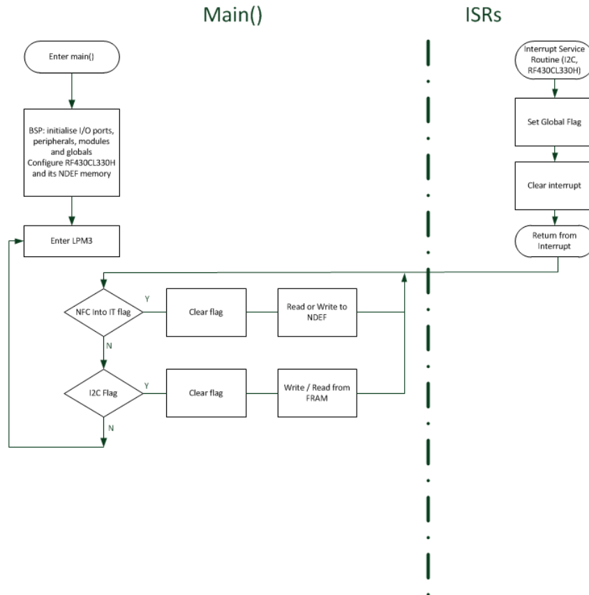
Figure 17. Software Flow Diagram
