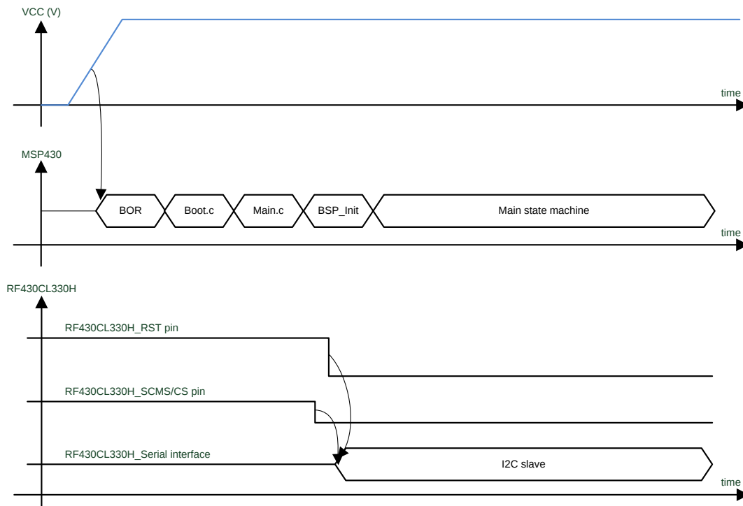
Figure 8. Hardware Power-Up Sequence
