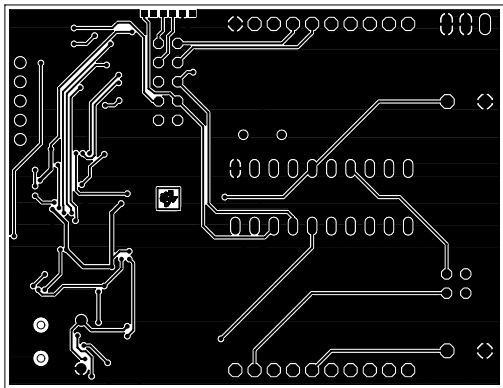
TIDM-LPBP-CONTACTLESSTEMPSENSE LaunchPad Silk Screen
