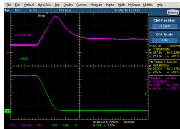
Figure 44. 5-0A load dump Vin=12V Vo=3.3V fsw=5MHz, Ch3 (purple): Vout, CH4(green): Io
