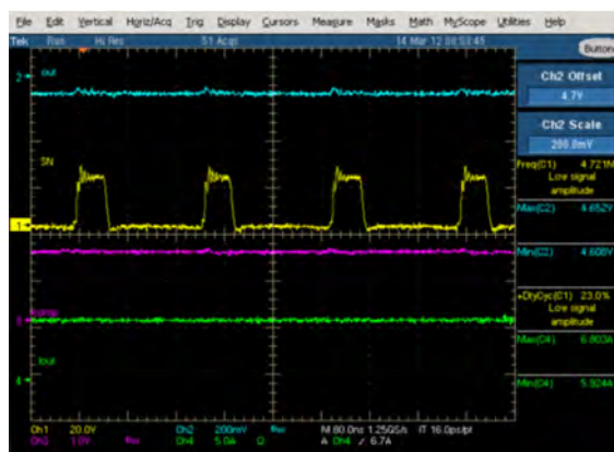
Figure 12. Sw node 4.7MHz operation 22Vin Vo=4.7V, Io=6A Ch1 (yellow): Switching node, Ch2 (blue): Vout Ch3 (purple): COMP, Ch4 (green): Load current.
