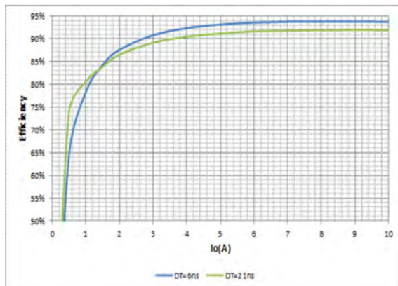
Figure 23. System efficiency improvement with different dead times Vin=12V Vo= 3.3V 1.25MHz
