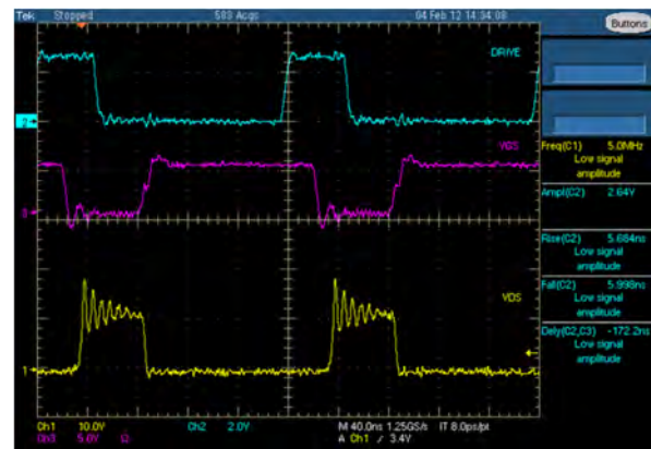
Figure 16. Low Gate drive and switching node, f_{sw}=5\text{MHz}
