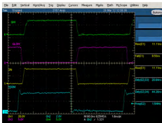
Figure 13. Gate drive and switching node f_{sw}=1.5\text{MHz} , no load
