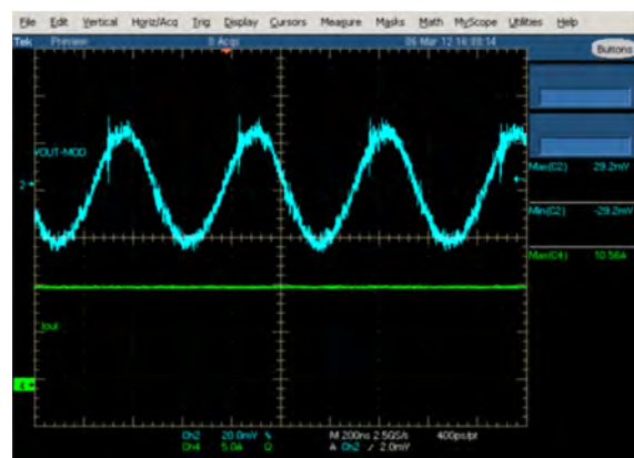
Figure 34. Ripple at 1MHz Vin=48V, Vo=30V, Io=10A Lo=1μH, Co=12μF ceramic +470μF electrolytic
