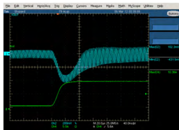
Figure 36. Transient response, 10A step down load 1MHz Vin=48V, Vo=30V, Io=10A Lo=1μH, Co=12μF ceramic
