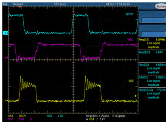
Figure 15. High Gate drive and switching node, f_{sw}=5\text{MHz}
