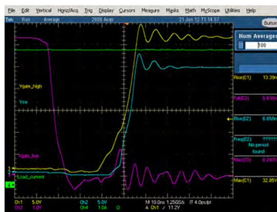
Figure 10. Detailed rise time plots, 24Vin, Vo=12V 6A out Ch1 (yellow): Vgate_high (measured on FET), Ch2 (blue): switching node Ch3 (purple): Vgate_low (measured on FET), Ch4 (green): Load current.
