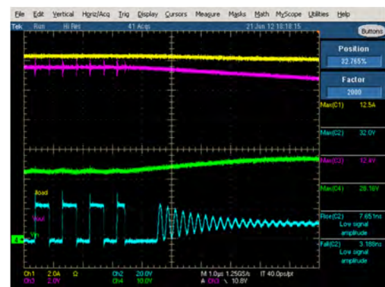
Figure 18. Expanded Current limit operation R_{ds\_on}=13\text{m}\Omega , R_{lim}=128\text{k}\Omega Ch1 (yellow): output current, Ch2 (blue): switching node Ch3 (purple): output voltage, Ch4 (green): input voltage.
