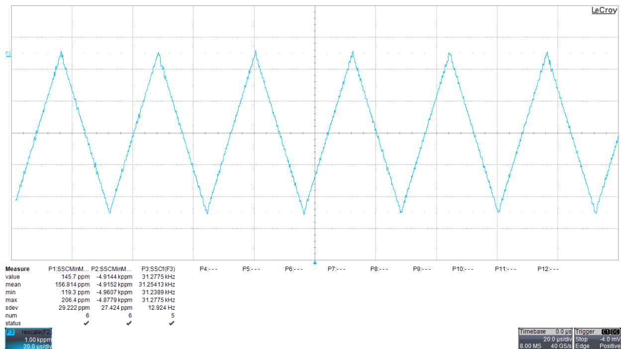
Figure 2. Spread Spectrum Clocking of TUSB9261-Q1. The SSC deviation was -4.9607kPPM and the modulation rate was 31.254kHz.
