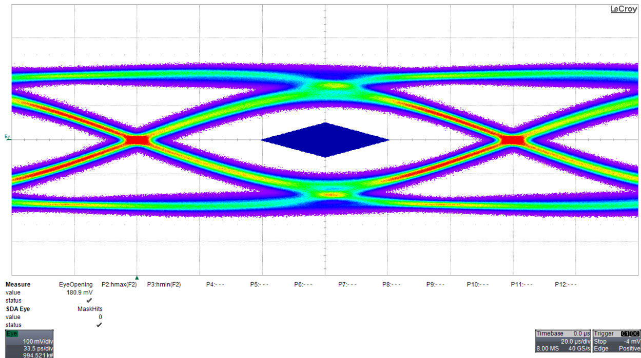
Figure 1. Tx eye diagram for TUSB9261-Q1. The eye height was 181mV.
