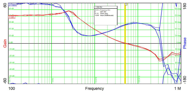
10Vin, 1.0Vout, 90A Load, BW=50.9kHz, PM=81deg, GM=25dB
