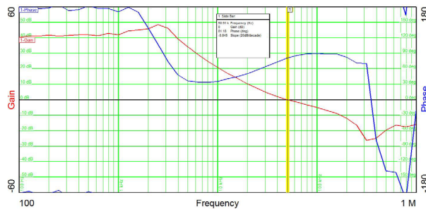
10Vin, 1.0Vout, No Load, BW=50.9kHz, PM=81deg, GM=25dB
