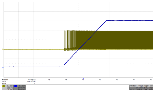
Turn-on, 10Vin, 1.0Vout (blue trace is Vout and yellow trace is switching waveform)
