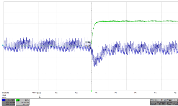
10Vin, 1.0Vout, 67.5A to 90A Load (blue trace is Vout, 10mV/div and green trace is step current 10A/div)
