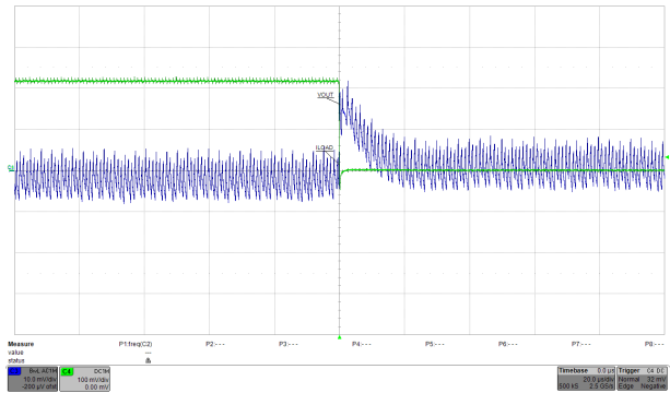
10Vin, 1.0Vout, 90A to 67.5 Load (blue trace is Vout, 10mV/div and green trace is step current 10A/div)
