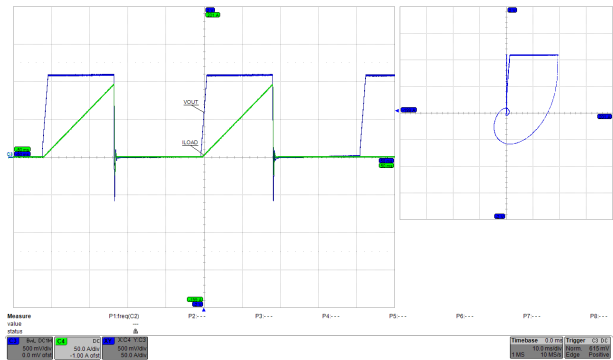
10Vin, 1.085Vout, Short circuit released
