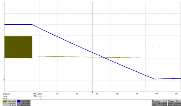
Turn-off, 10Vin, 1.0Vout (blue trace is Vout and yellow trace is switching waveform)
