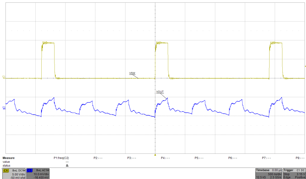
10Vin, 1.0Vout, 90A load, SW node and Vout
