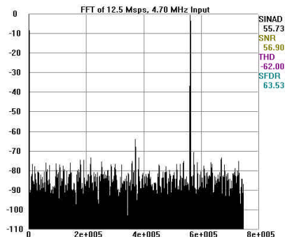
Figure 7. The Flat-Top windowing function yields slightly improved dynamic performance measurements over the Hanning function.
