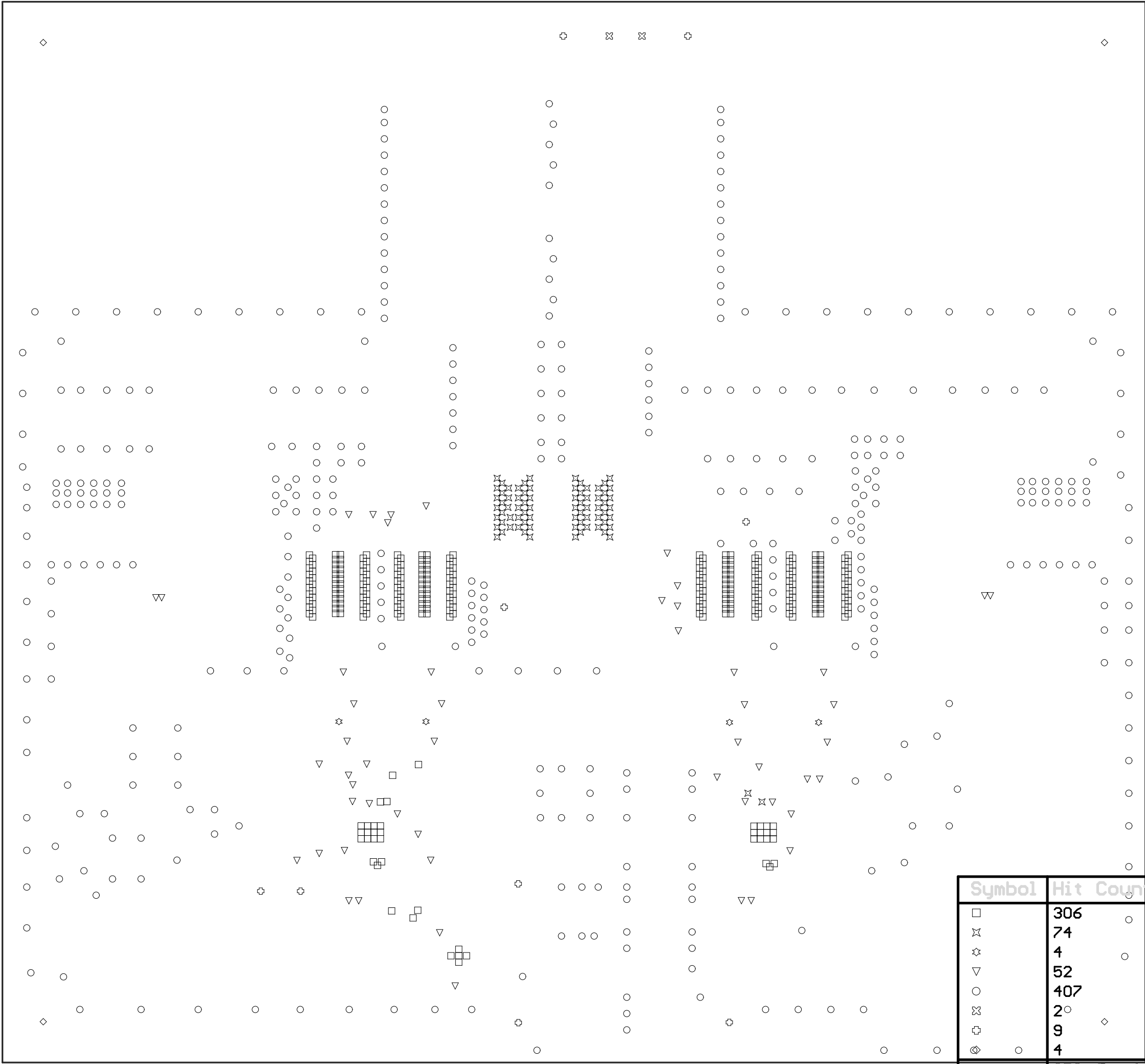
Drill Table
