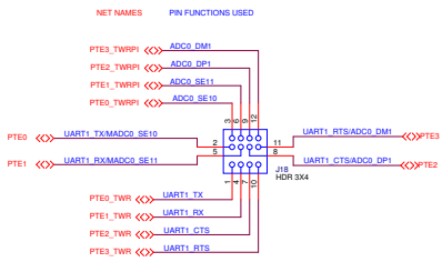
UART1/ADC TWRPI/TWR_ELEV_Select
