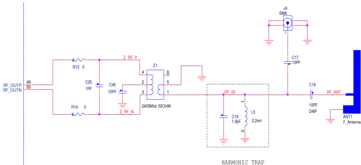
Figure 3-4. TWR-KW24D512 RF Circuitry
