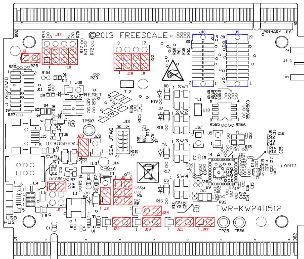
Figure 3-1. TWR-KW2x
