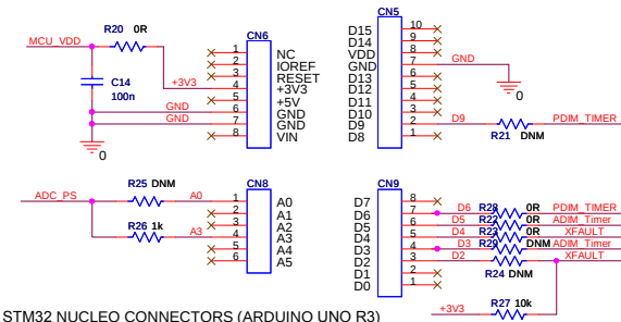
STM32 NUCLEO CONNECTORS (ARDUINO UNO R3)
