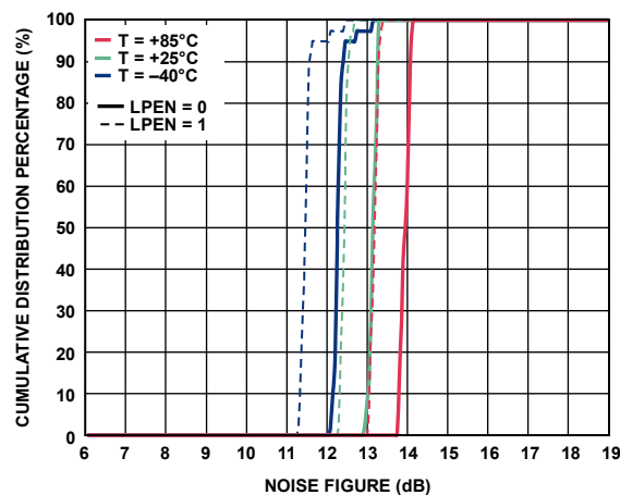
Figure 31. Noise Figure
