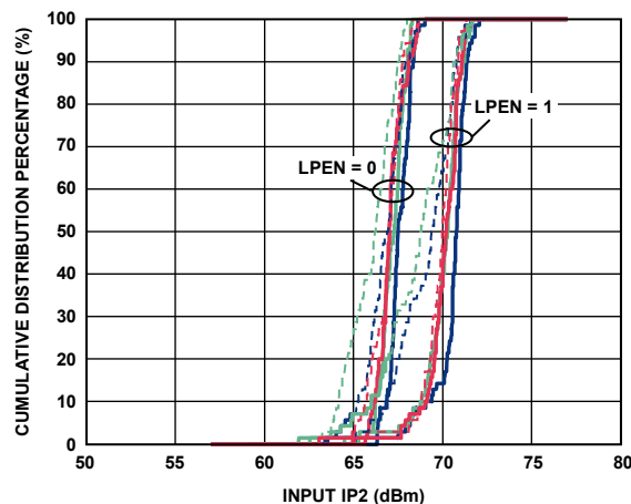
Figure 30. Input IP2
