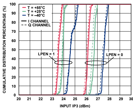
Figure 28. Input IP3
