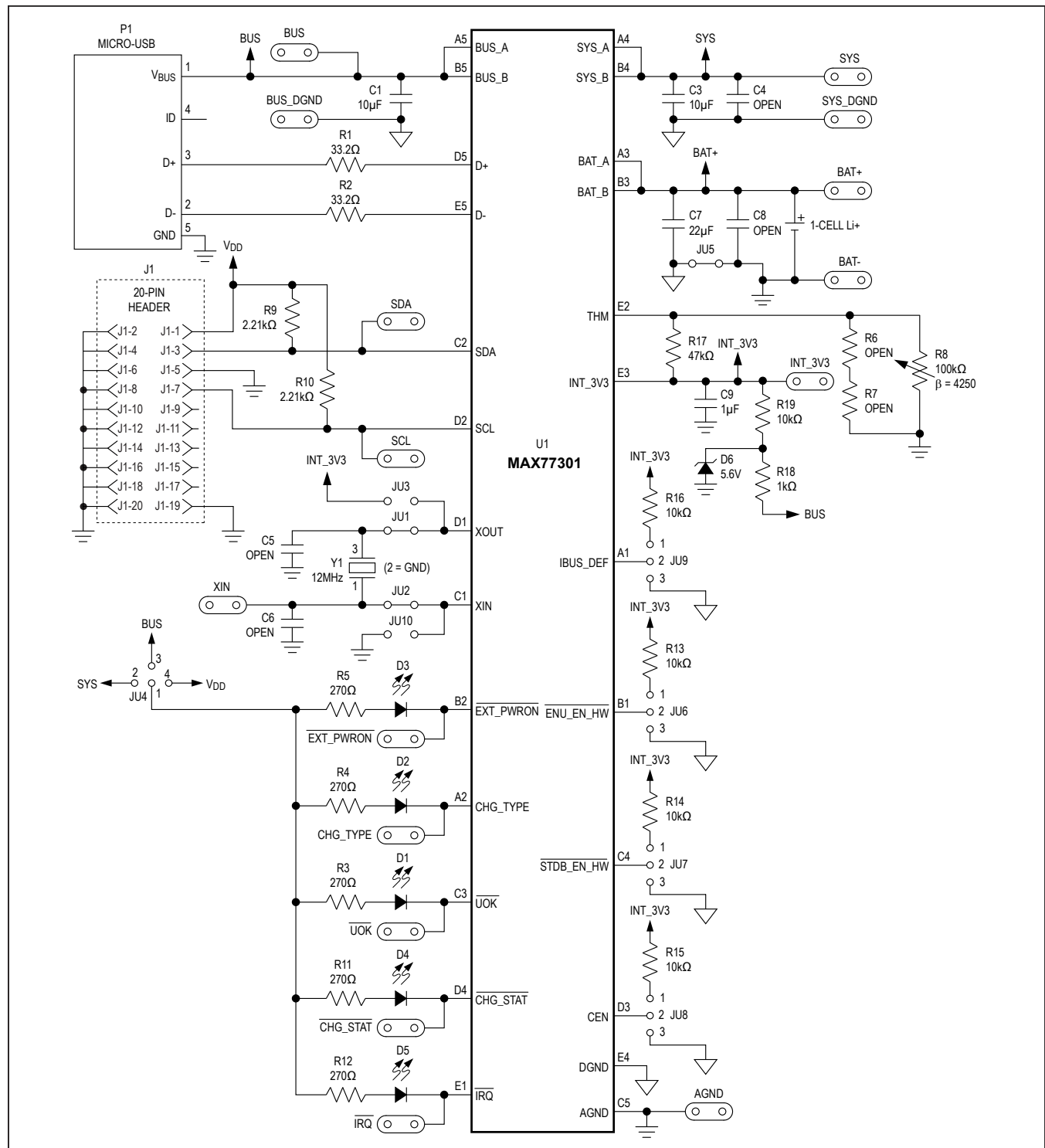
Figure 9. MAX77301 EV Kit Schematic
