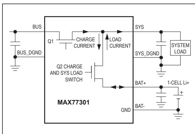
Figure 1. Smart Power Selector
