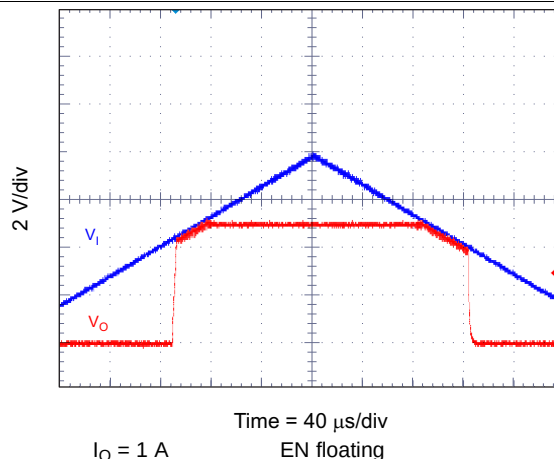
Figure 62. Low-Dropout Operation
