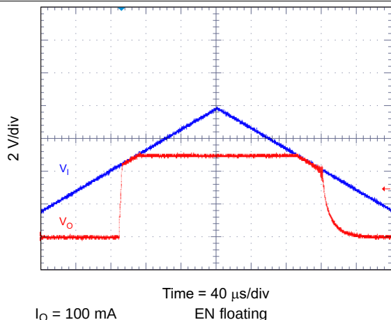
Figure 61. Low-Dropout Operation
