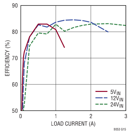
Efficiency vs Load Current, V_{OUT} = -12\text{V} , BIAS tied to LTM8053 GND
