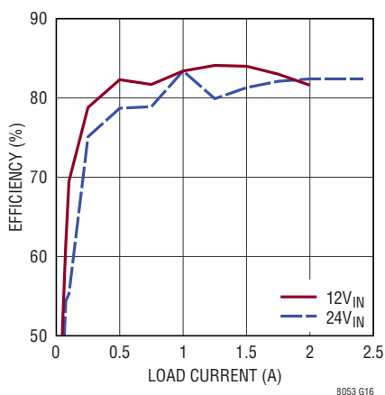
Efficiency vs Load Current, V_{OUT} = -15\text{V} , BIAS tied to LTM8053 GND
