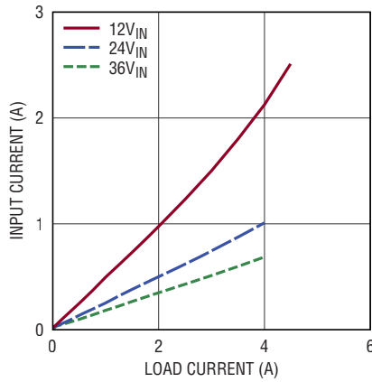
Input vs Load Current V_{OUT} = -5\text{V} , BIAS tied to LTM8053 GND
