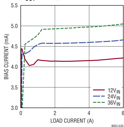
BIAS Current vs Load Current V_{OUT} = 1.5\text{V} , BIAS = 5V
