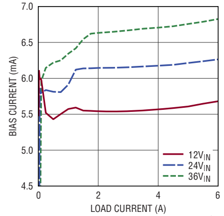
BIAS Current vs Load Current V_{OUT} = 3.3V , BIAS = 5V
