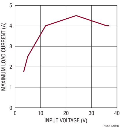
Maximum Load Current vs V_{IN} . BIAS Open
