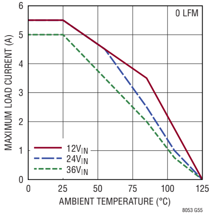
Derating, V_{OUT} = 5\text{V} , BIAS = 5V, DC1934A Demo Board
