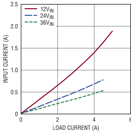
Input vs Load Current V_{OUT} = -3.3\text{V} , BIAS tied to LTM8053 GND
