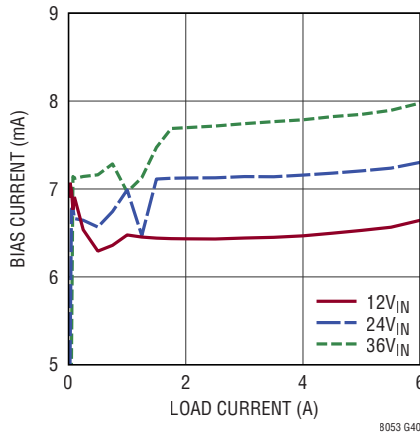
BIAS Current vs Load Current V_{OUT} = 5V , BIAS = 5V
