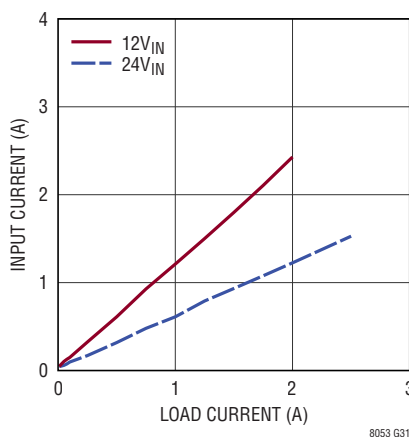
Input vs Load Current V_{OUT} = -12\text{V} , BIAS tied to LTM8053 GND
