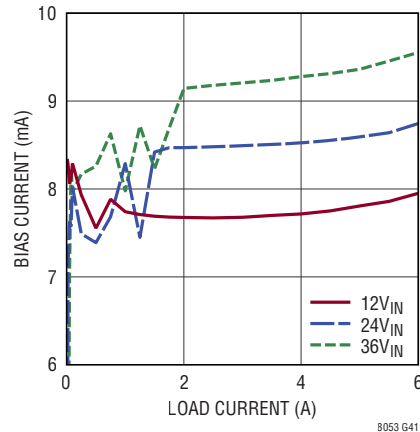
BIAS Current vs Load Current V_{OUT} = 8V , BIAS = 5V
