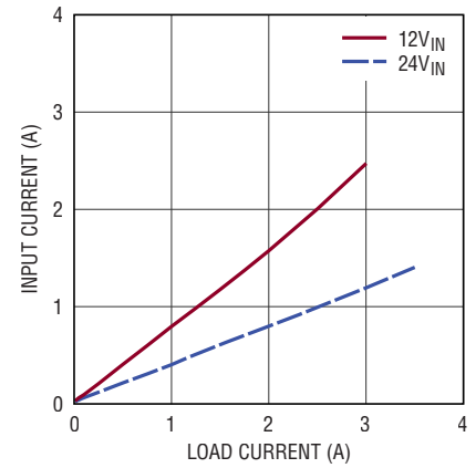
Input vs Load Current V_{OUT} = -8\text{V} , BIAS tied to LTM8053 GND
