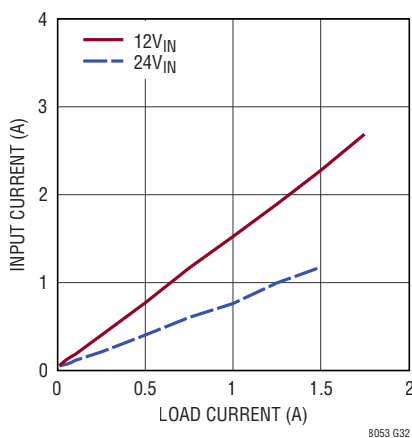
Input vs Load Current V_{OUT} = -15\text{V} , BIAS tied to LTM8053 GND
