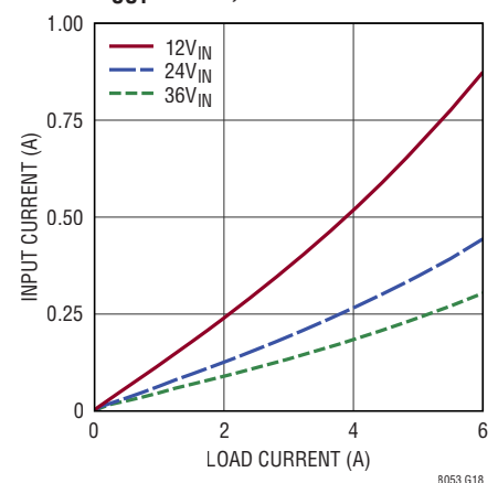
Input vs Load Current V_{OUT} = 1.2\text{V} , BIAS = 5V
