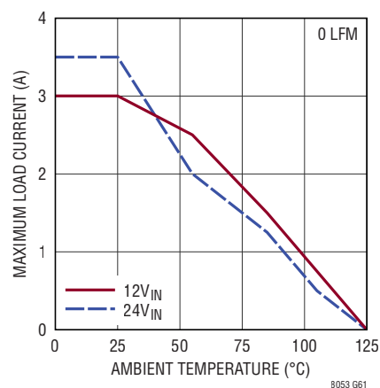
Derating, V_{OUT} = -8\text{V} , BIAS tied to LTM8053 GND, DC1934A Demo Board
