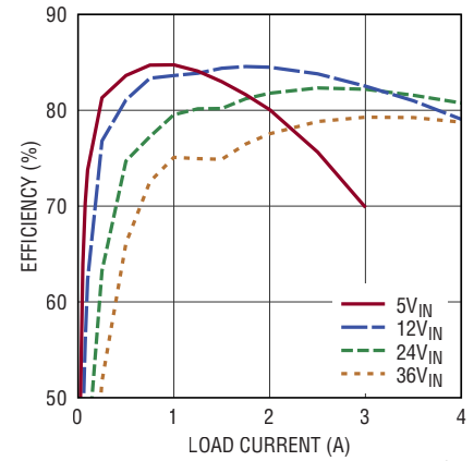
Efficiency vs Load Current, V_{OUT} = -3.3\text{V} , BIAS tied to LTM8053 GND
