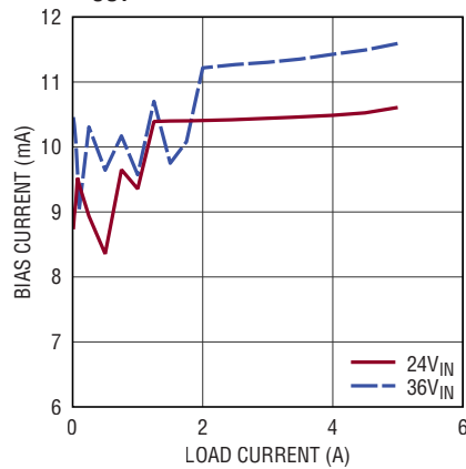
BIAS Current vs Load Current V_{OUT} = 15V , BIAS = 5V
