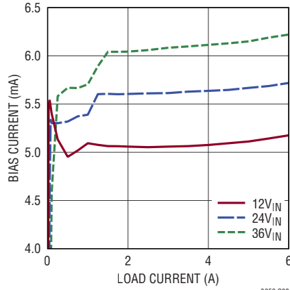
BIAS Current vs Load Current V_{OUT} = 2.5V , BIAS = 5V
