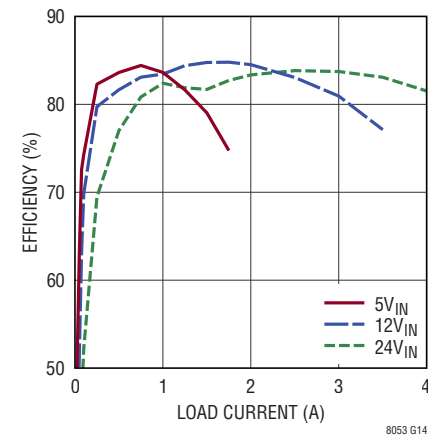
Efficiency vs Load Current, V_{OUT} = -8\text{V} , BIAS tied to LTM8053 GND
