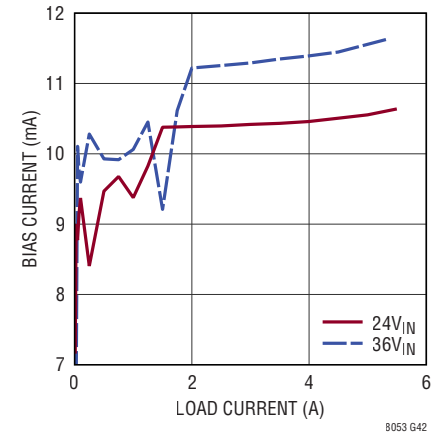
BIAS Current vs Load Current V_{OUT} = 12V , BIAS = 5V
