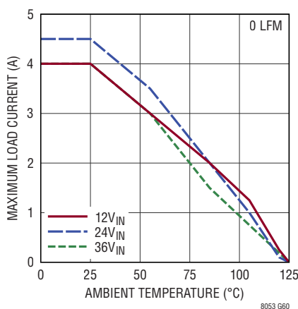
Derating, V_{OUT} = -5\text{V} , BIAS tied to LTM8053 GND, DC1934A Demo Board
