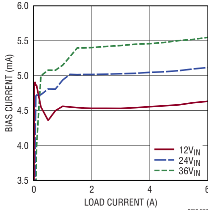
BIAS Current vs Load Current V_{OUT} = 2V , BIAS = 5V
