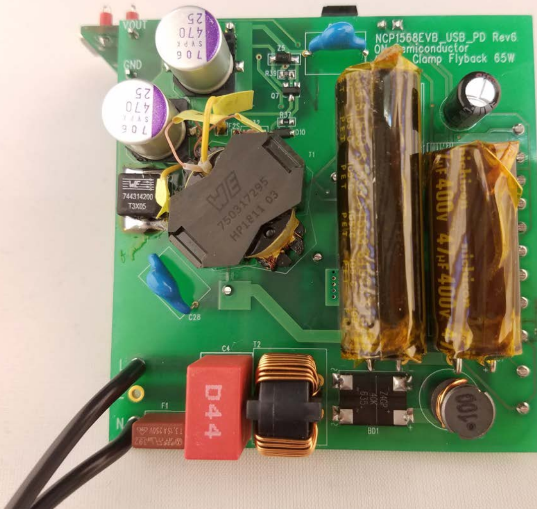
Figure 1 Top View of the Demo Board
