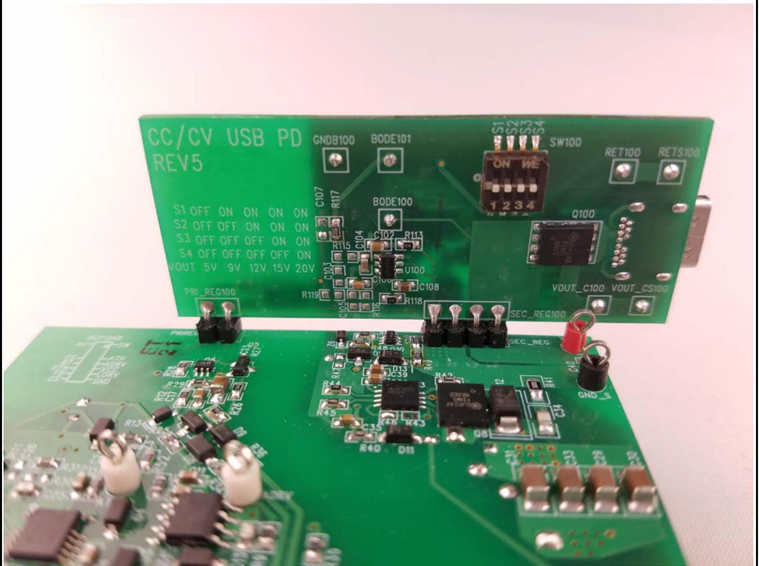
Figure 3 Bottom View of Daughter Card
