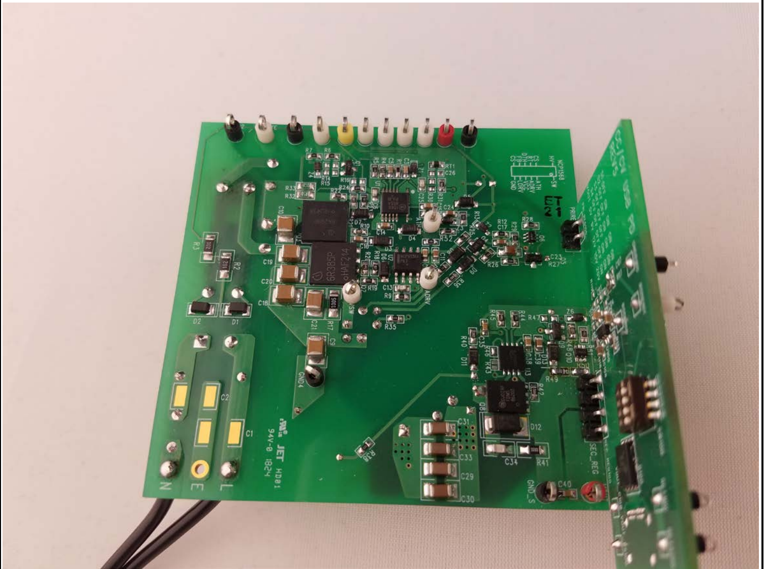
Figure 2 Bottom View of the Demo Board
