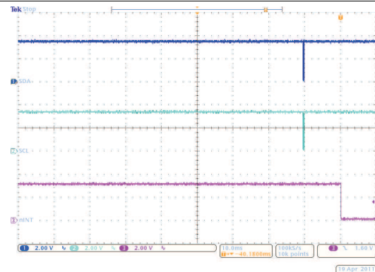
Figure 18. Kickback Voltage Measurement Timing Time from ACQ Bit Set to ACQC Interrupt Received
