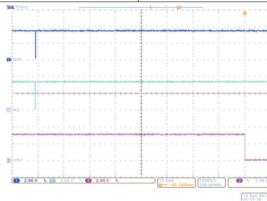
Figure 19. Kickback Voltage Measurement Timing Time from ACQ Bit Set to ACQC Interrupt Received
