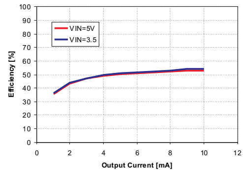
Figure 48. VB DCDC Efficiency
