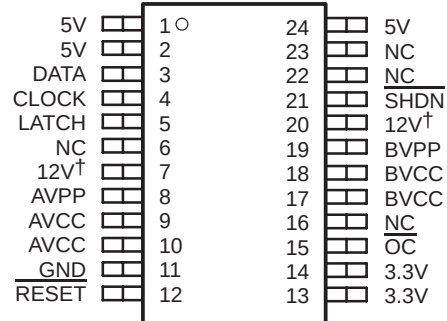
TPS2223, TPS2224 DB OR PWP PACKAGE (TOP VIEW)
