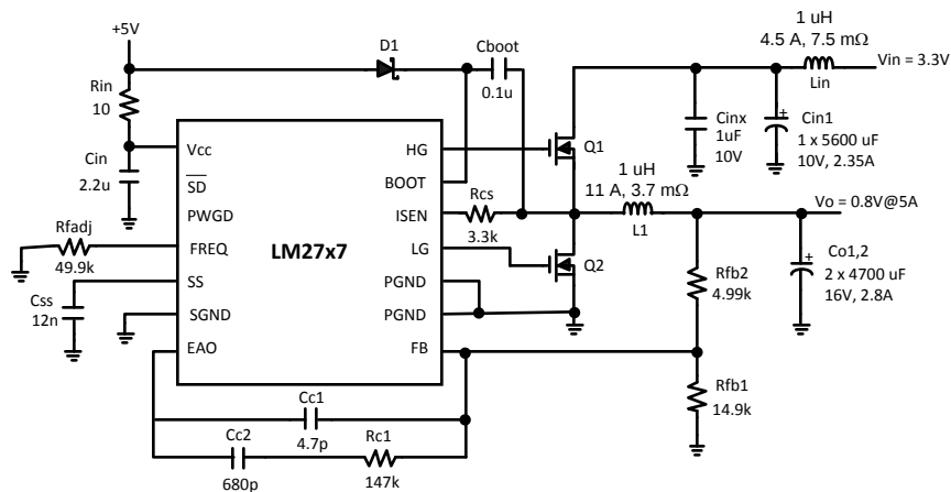
Figure 28. 3.3V to 0.8V, 5A, 500kHz
