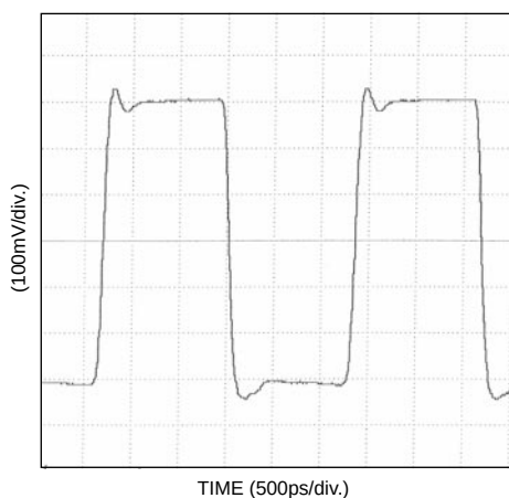
Figure 6. Output Waveform (750Mbps w/ I_{MOD} \sim 50\text{mA} , +3.3V)
