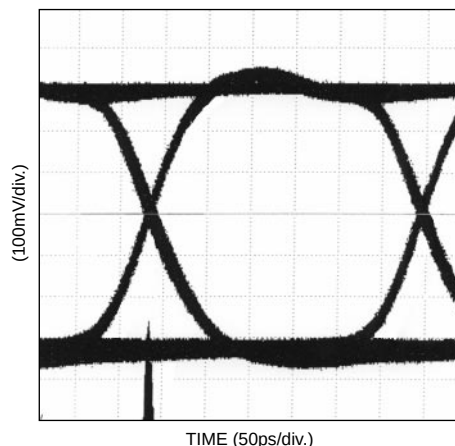
Figure 7. Output Waveform (3.2Gbps w/ I_{MOD} \sim 50\text{mA} , +3.3V)
