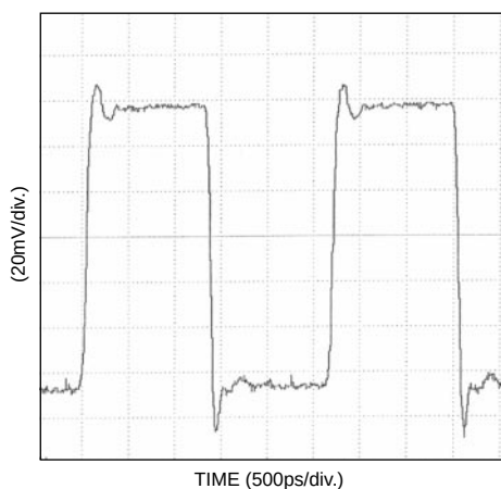
Figure 2. Output Waveform (750Mbps w/ I_{MOD} \sim 10mA , +3.3V)
