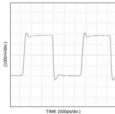
Figure 4. Output Waveform (750Mbps w/ I_{MOD} \sim 30mA , +3.3V)
