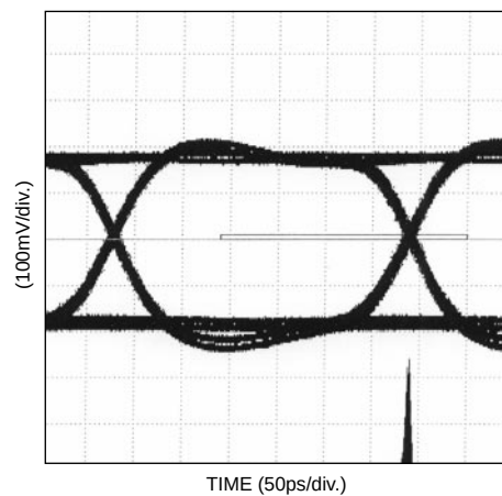
Figure 5. Output Waveform (3.2Gbps w/ I_{MOD} \sim 30mA , +3.3V)
