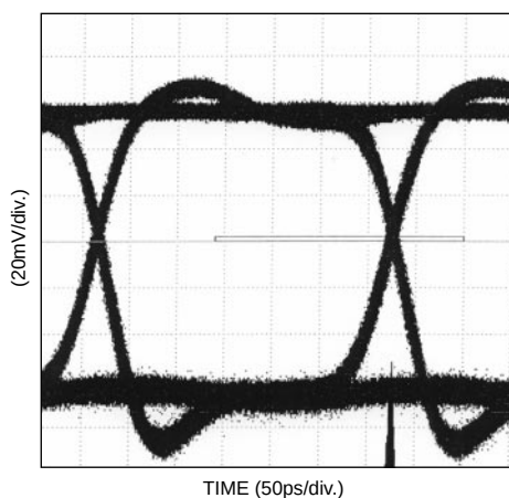
Figure 3. Output Waveform (3.2Gbps w/ I_{MOD} \sim 10mA , +3.3V)
