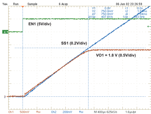
Figure 21. Start-Up Waveforms
