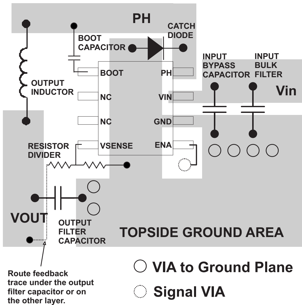
Figure 9. Design Layout
